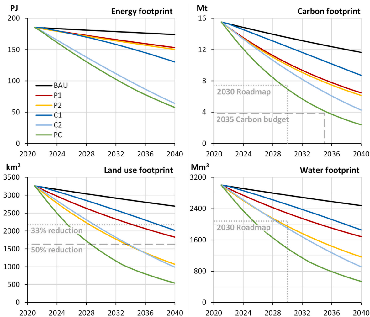
Fig. 5. Environmental impacts of the UK clothing economy from 2021 to 2040 in the six scenarios for energy (petajoules), carbon (megatonnes of CO 2 e), land use (square kilometers) and water (million cubic metres). Existing, related, or proposed targets are shown in grey where applicable (see main text for details).
