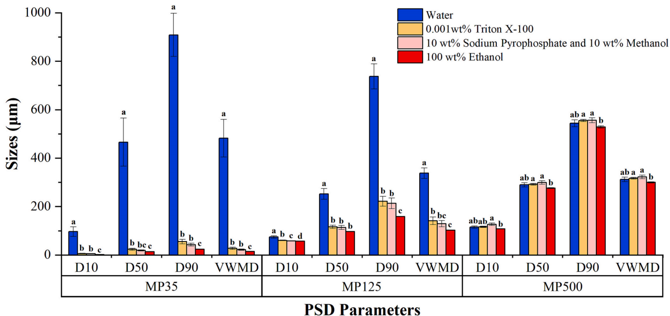
Fig. 4. The particle size distribution parameters of different size fractions of MP particles measured with different dispersants. Data are means ( \pm SD, n = 3). The one-way ANOVA tests reveal significant difference between treatments ( p < 0.03 ). Superscript letters indicate significant differences ( p < 0.05 ) between the treatments.
