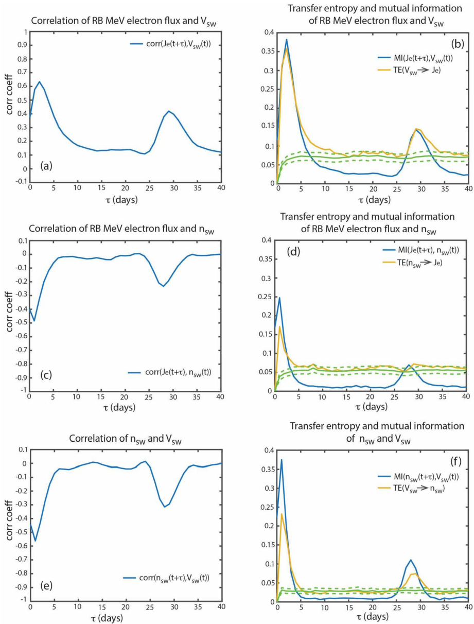
Fig. 12 (adapted from Wing et al. 2016) (a) Correlation coefficient of [j_{e,GEO}(t + \tau), V_{sw}(t)] . (b) \text{MI}(j_{e,GEO}(t + \tau), V_{sw}(t)) (blue) and \text{TE}(j_{e,GEO}(t + \tau), V_{sw}(t)) (yellow). The transfer of information from V_{sw} to j_{e,GEO} ( \text{TE}(V_{sw} \rightarrow j_{e,GEO}) ) peaks at \tau_{\max} = 2 days. (c) Correlation coefficient of [j_{e,GEO}(t + \tau), n_{sw}(t)] . (d) \text{MI}(j_{e,GEO}(t + \tau), n_{sw}(t)) (blue) and \text{TE}(j_{e,GEO}(t + \tau), n_{sw}(t)) (yellow). The transfer of information from n_{sw} to j_{e,GEO} ( \text{TE}(n_{sw} \rightarrow j_{e,GEO}) ) peaks at \tau_{\max} = 1 day. (e) Correlation coefficient of [n_{sw}(t + \tau), V_{sw}(t)] . (f) \text{MI}(n_{sw}(t + \tau), V_{sw}(t)) (blue) and \text{TE}(n_{sw}(t + \tau), V_{sw}(t)) (yellow). The solid and dashed green curves are the mean and 3\sigma from the mean of the noise. The transfer of information from V_{sw} to n_{sw} ( \text{TE}(V_{sw} \rightarrow n_{sw}) ) peaks at \tau_{\max} = 1 day
