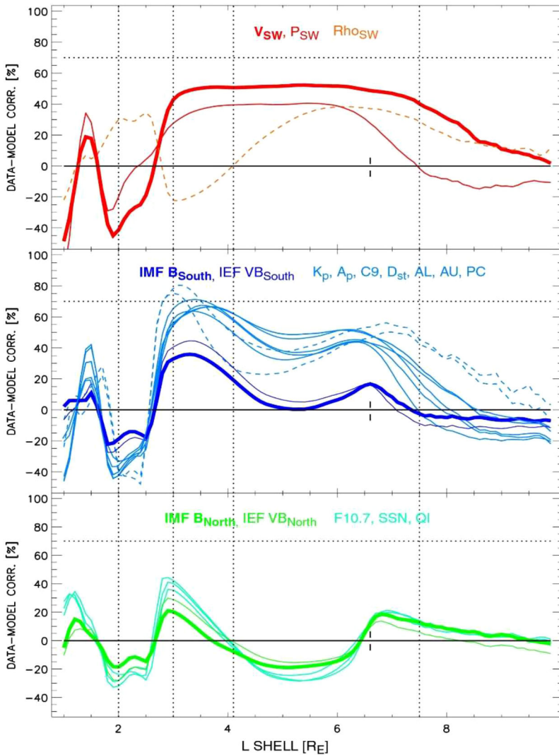
Fig. 14 (Fig. 3 from Vassiliadis et al. 2005) Data-model correlation C(l) ( L ) from Equation (5.1) for 17 interplanetary/magnetospheric variables. (top) Solar wind plasma parameters V_{SW} (red thick line), P_{SW} (red thin line), and n_{SW} (orange dashed line) represent the hydrodynamic aspects of the solar wind–magnetosphere interaction. (middle) Interplanetary inputs B_{South} (blue thick line) and V_{SW}B_{South} (blue thin line) and magnetic indices K_p , A_p , C9 , Dst , AL , AU , and PC (light blue lines) represent the effects of magnetic reconnection. AL and AU are denoted by dashed lines. (bottom) Interplanetary inputs B_{North} (green thick line), V_{SW}B_{North} (green thin line), and solar wind quasi invariant QI as well as solar variables F10.7 and SSN (cyan lines) show the effect of electron losses
