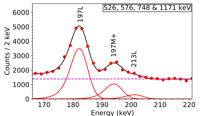
FIG. 6. A fit (black solid line) to a portion of the electron energy spectrum, gated on the 526-, 576-, 748-, and 1171-keV \gamma rays feeding the 548 keV 2_2^+ state in ^{182}\text{Hg} . The visible peaks stem from the L - and M+ -ICE of the 197-keV transition and the L -ICE of the 213-keV transition. A contribution from asymmetric Gaussian functions is plotted in solid red lines and the constant background is shown by the dashed purple line.
