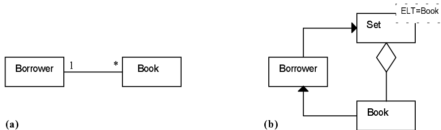
Figure 1: Direct encoding of 1:M relationship
