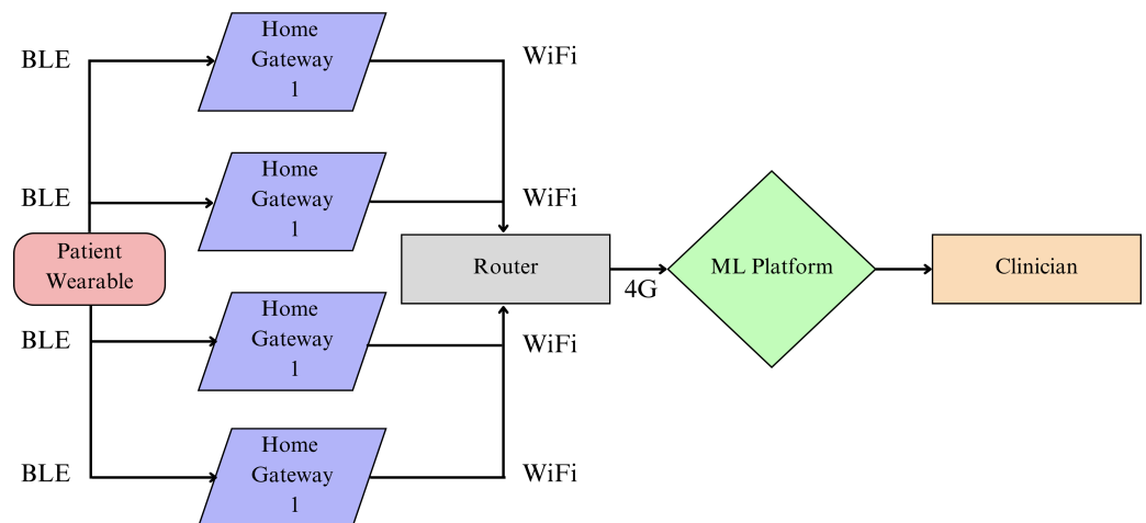
Figure 13. Vesta platform overview. Reprinted with permission from [72].
