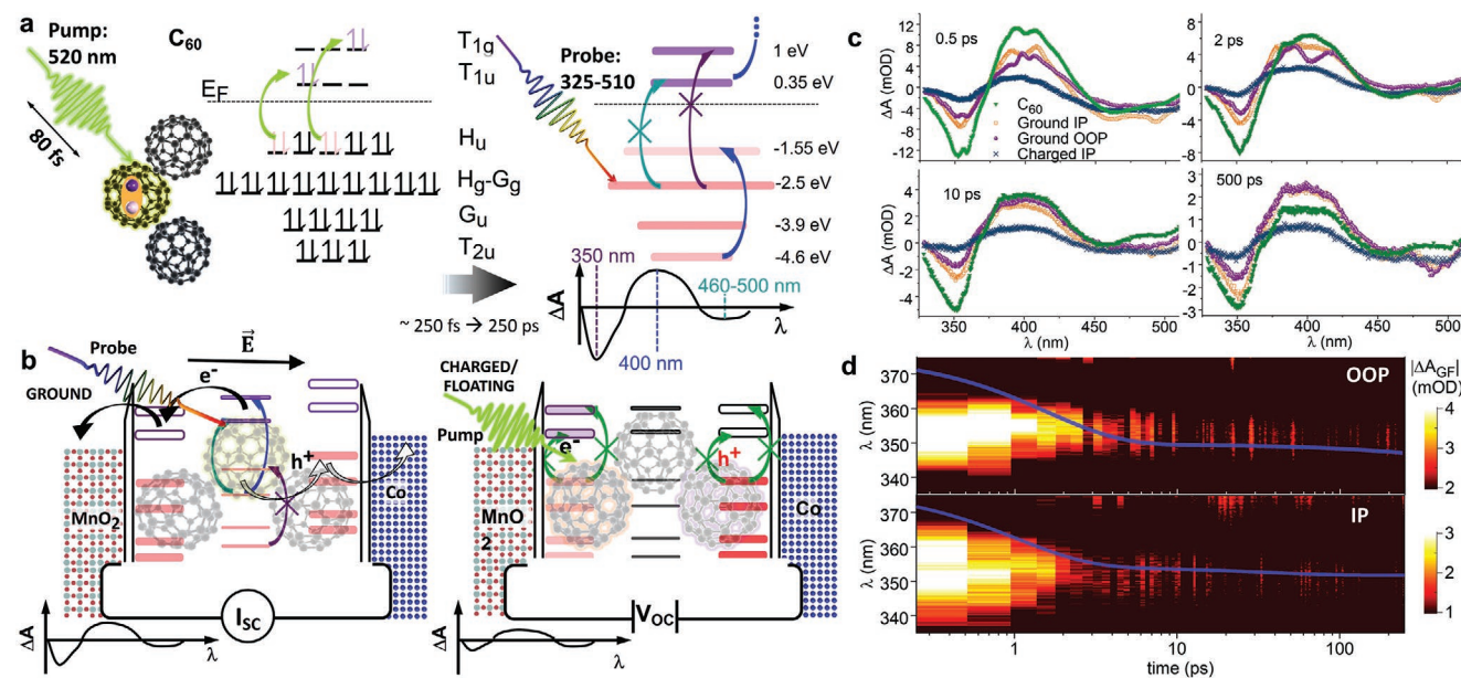
Figure 3. Time-resolved TA spectroscopy in a magneto-photovoltaic structure. Schematic of TA spectroscopy in a pristine C_{60} film a) and in a MnO_2/Co spin photovoltaic device b) Note that energies are approximate and levels will broaden in proximity to the interfaces. [13] a) Pump irradiation at 520 nm generates excitons by electron promotion from HOMO (Hu) to LUMO (T1u) and LUMO+1 (T1g). The T1u, T1g occupancy reduces the probe absorbance at 350 and 460 nm (HOMO-1 Hg-Gg \rightarrow T1g, T1u), whereas holes at the HOMO and re-excitation of LUMO states allow for increased absorption at 400 nm. b) In a ground device, changes in absorption ( \Delta A ) are small because carriers are driven to the electrodes by the dipolar electric fields at the interfaces (b-left). In floating devices, the pump cannot excite molecules already charged due to electron accumulation/trapping at the interface. \Delta A is therefore also small, since the probe does not measure strong changes after excitation (b-right). c) TA spectroscopy in the 330–510 nm range measured 0.5 ps, 2 ps, 10 ps, and 500 ps after excitation in a C_{60} film and a Co/ C_{60} / MnO_2 junction in different states. d) Difference in the TA spectrum at 330–380 nm between the charged and the grounded device after an OOP (top) or IP magnetic field (bottom). The blue line insets show |\Delta A_{GF}| fit to a double exponential decay with the main time constants of 1.3 \pm 0.2 ps; 40 \pm 10 ps (OOP) or 2 \pm 0.3 ps; 400 \pm 200 ps (IP).
