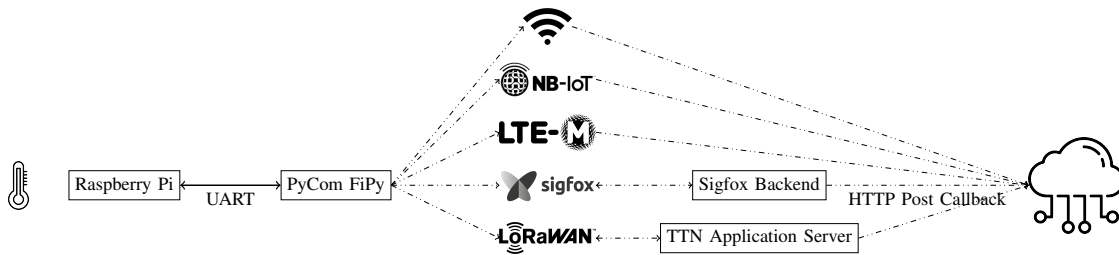
Fig. 3: Block diagram of current experimental setup.
