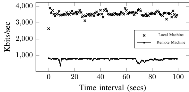
Fig. 6: Bandwidth results using iperf when running on local network and cloud.
