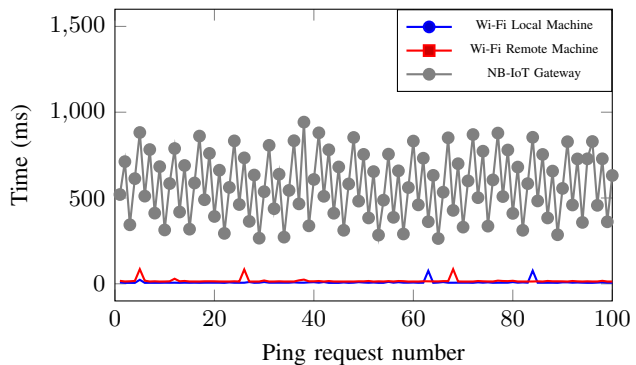
Fig. 5: Latency results for pingging a local machine and cloud machine via Wi-Fi and gateway via NB-IoT network.
