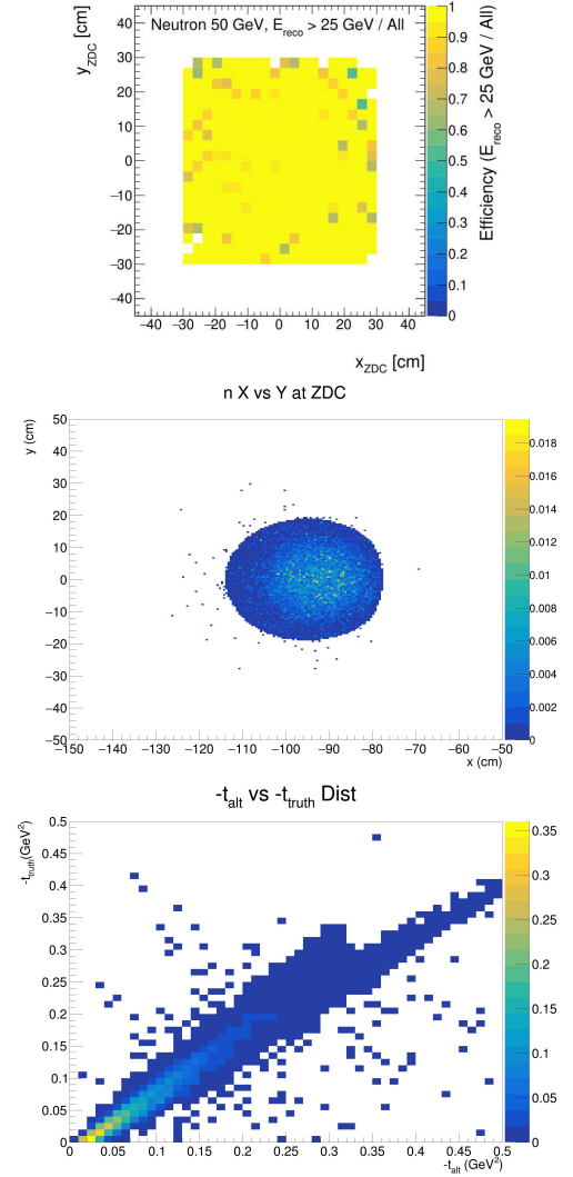
Figure 26: (top) ZDC detection efficiency for neutrons in its local coordinate system. (middle) Detection distribution of neutron hits in the ZDC for meson structure function processes without the beam pipe blocking contribution. z -axis reflects the normalized yield. (bottom) Reconstructed t versus true t , where t is reconstructed as from the baryon information, t_{alt} = (p_p - p_n)^2 , which is reliable with a resolution of < 0.025 GeV 2 .
