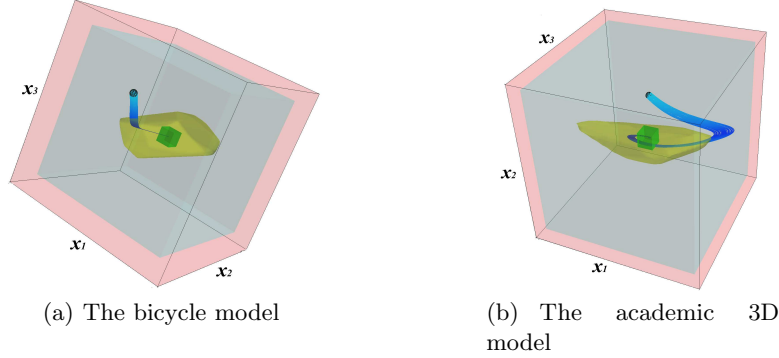
Fig. 12. Learned and verified NN controllers and barriers for Example 4 and 5: for both cases, the innermost cube (green) represents the initial set, the outermost cube (pink) represents the system domain, and the space between the outermost and the middle cube (grey) is the unsafe region; the irregular surface (yellow) surrounding the innermost cube is the zero-level set of synthesized NN barrier; the curves (blue) approaching the origin are simulated system trajectories
