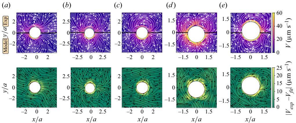
Figure 3. Top row: comparison between the experimental flow fields v_{exp} (top half of each panel) and fits to the Brinkman approximation v_{fit} (bottom half) for different Pe , with fit parameters b_1, b_2 : (a) Pe = 26 ( b_2/b_1 = -0.529 ), (b) Pe = 38 ( b_2/b_1 = -0.001 ), (c) Pe = 62 ( b_2/b_1 = 0.191 ), (d) Pe = 130 ( b_2/b_1 = 4.915 ) and (e) Pe = 204 ( b_2/b_1 = 0.175 ). Depending on the b_2/b_1 ratio, we note a shift of the vortex pair towards the droplet anterior, and a bistability of dipolar and quadrupolar patterns for large droplets. Bottom row: residual flow fields, |v_{exp} - v_{fit}| .
