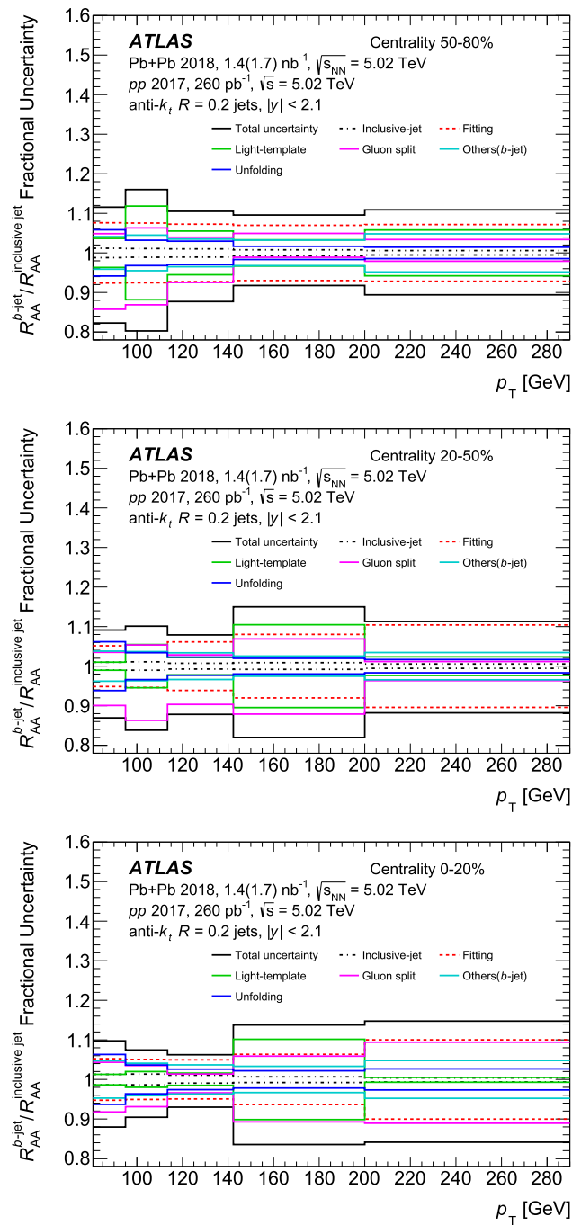
Fig. 6 Relative size of systematic uncertainties of the ratio R_{AA}^{b-jet} / R_{AA}^{inclusive jet} shown for the most relevant components, as a function of jet p_T for 50–80% (top), 20–50% (middle), and 0–20% (bottom) centrality Pb+Pb collisions
