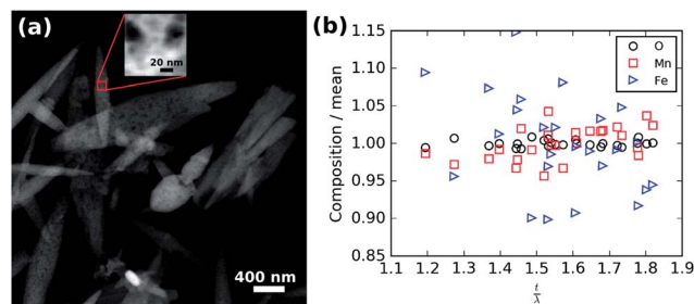
Fig. 7 (a) Overview HAADF image showing the region from which the EELS data were collected (red box). Inset HAADF signal collected during EELS acquisition. (b) Normalised relative composition versus thickness.
