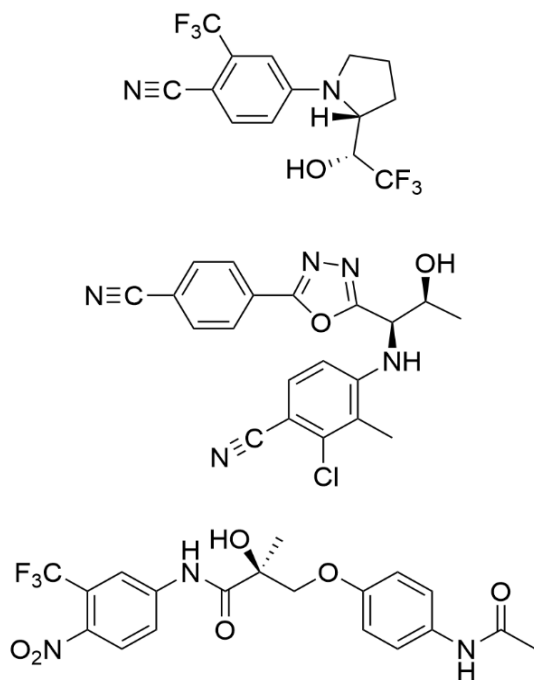
Figure 1. The structures of ligandrol (top), RAD-140 (centre) and andarine (bottom) - a common SARMs used in both therapeutic and sports doping settings.
