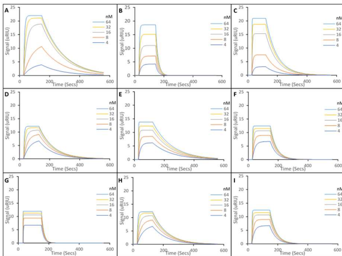
Figure 2: Representative SPR curves showing rebinding of target and non-target SARMs to the immobilised nanoMIPs. Five concentrations of analyte in PBST. (A) Andarine binding to Andarine-imprinted nanoMIPs; (B) Ligandrol binding to Ligandrol-imprinted nanoMIPs; (C) RAD-140 binding to RAD-140-imprinted nanoMIPs; (D) Ligandrol binding to Andarine-imprinted nanoMIPs; (E) Andarine binding to Ligandrol-imprinted nanoMIPs and (F) Andarine binding to RAD-140-imprinted nanoMIPs; (G) RAD-140 binding to Andarine-imprinted nanoMIPs; (H) RAD-140 binding to Ligandrol-imprinted nanoMIPs and (I) Ligandrol binding to RAD-140-imprinted nanoMIPs.
