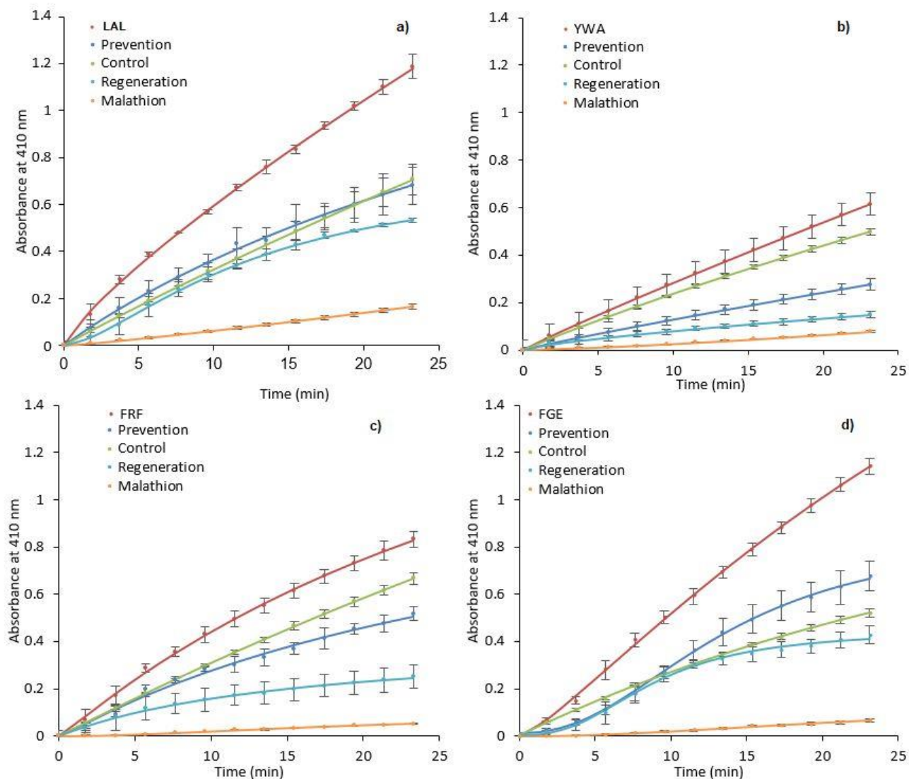
Figure 4: Prevention and regeneration of AChE by MIPs. LAL-MIP (a), YWA-MIP (b), FRF-MIP (c) and FGE-MIP (d)) following inhibition from Malathion. Error bars indicate SD.
