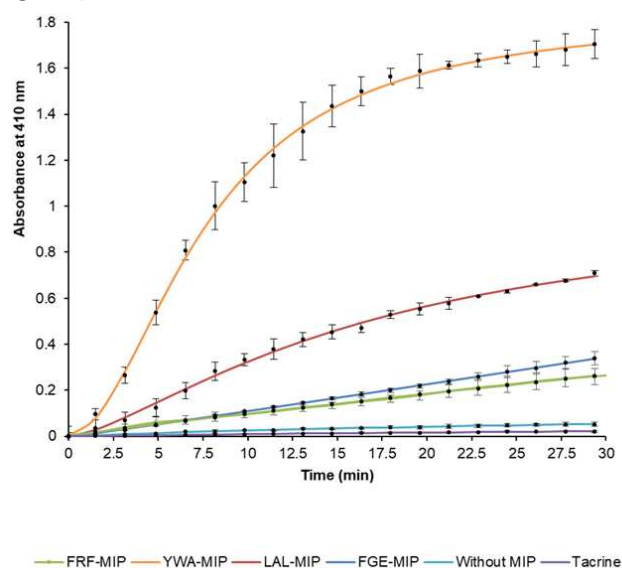
Figure 3: Hydrolysis of ATCh by EeAChE in the presence of select epitope-imprinted MIPs. Generation of thiocholine by AChE ( 25.0 \text{ mU mL}^{-1} ) in the presence of epitope-imprinted MIPs ( 0.7 \text{ mg mL}^{-1} ) or tacrine ( 50 \text{ nM} ); error bars indicate SD values. N=3 .
