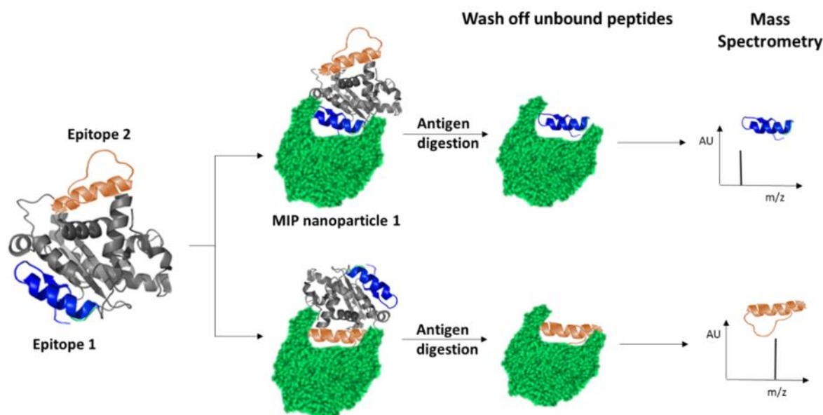
Figure 1: Schematic highlighting the principle of identification of peptide sequences exposed on protein surfaces using molecular imprinting and mass spectrometry.
