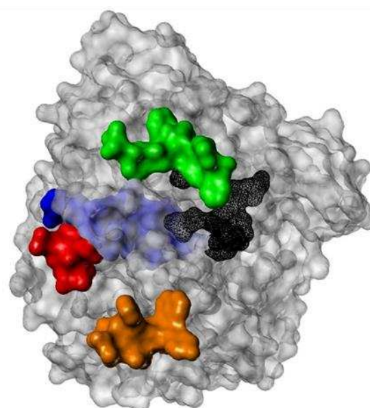
Figure 2: The relative positions of the four identified epitope sequences. LALQWVQDNIHFFGGNPK (red), FRFSFVPV (green), QVTIFGESAGAASVGMHLLSPDSRPK (blue), and YWANFAR (orange) are shown on the surface of EeAChE, as well as the location of the active site (black).
