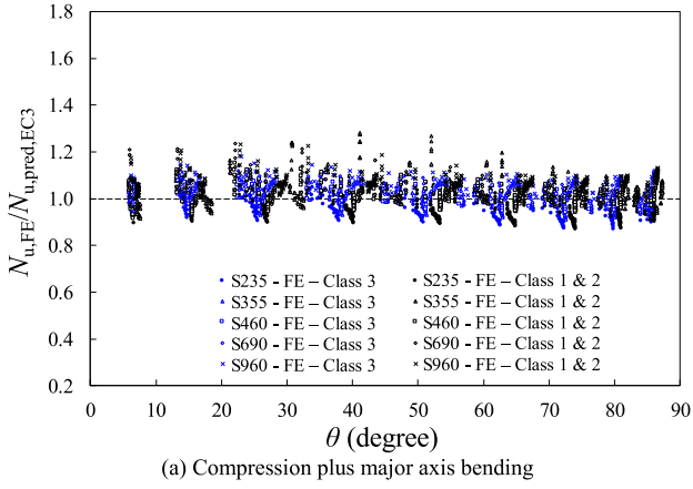
Fig. 9. Comparison of FE and test results with EC3 resistance predictions for NSS and HSS non-slender welded I-section beam-columns under combined loading.
