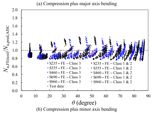
Fig. 10. Comparison of FE and test results with AISC resistance predictions for NSS and HSS non-slender welded I-section beam-columns under combined loading.
