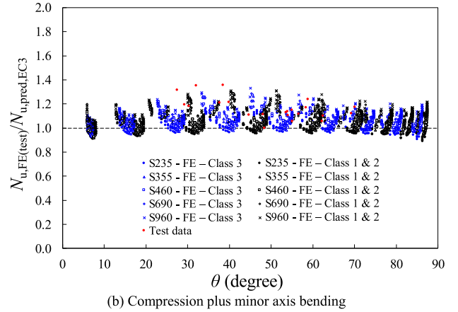
Fig. 9. Comparison of FE and test results with EC3 resistance predictions for NSS and HSS non-slender welded I-section beam-columns under combined loading.
