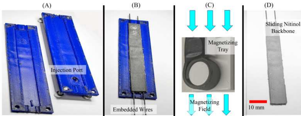
Figure 4: The key steps in the process of fabrication. (A) A mold is 3D printed in Poly(lactic acid). The injection port can be seen here. (B) 0.75 mm diameter nitinol wires are embedded lengthways and doped silicone is injected and cured. (C) The specimen is demolded, wrapped around a magnetizing tray (shown in grey) of specific bending radius and exposed to a saturating magnetizing field, shown here as turquoise arrows. (D) 0.5 mm diameter nitinol wires are inserted to act as the sliding backbone.
