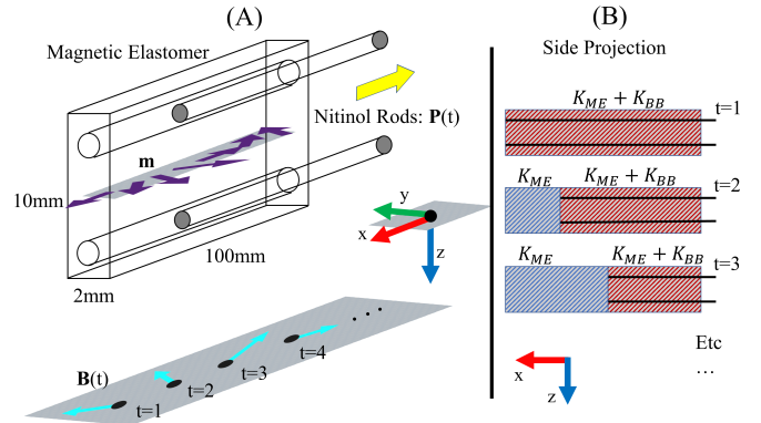
Figure 2: Schematic of the underlying design and actuation strategy for arbitrary time steps ( t = 1, 2, 3.. ). (A) The elastomer is magnetized ( \mathbf{m} ), shown as purple arrows, in the x - y plane (shown in grey) in a spatially sinusoidal fashion along the length of the x -axis. A temporally sinusoidal actuating field ( \mathbf{B}(t) , turquoise arrows) is applied (also in the x - y plane), as the nitinol rod backbone is withdrawn ( \mathbf{P}(t) , yellow arrow). (B) This controlled augmentation of the unconstrained, and therefore lower stiffness, length of the VSR allows higher strain energy states to be achieved. K_{ME} and K_{BB} are the elastic stiffness of the magnetic elastomer and the nitinol backbone, respectively.
