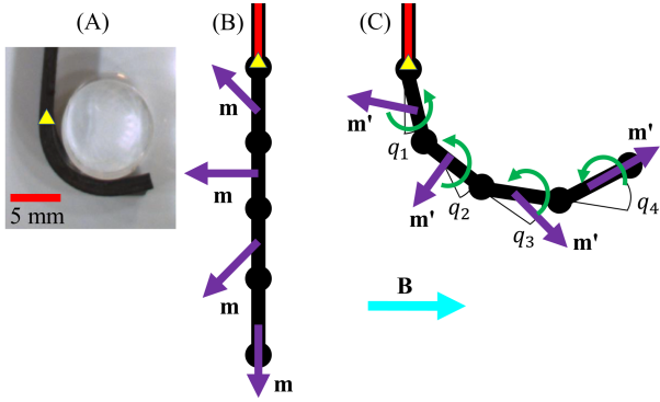
Figure 3: (A) A representative pose of the VSR with the tip location of the sliding nitinol backbone indicated by the yellow triangle and the backbone supported region shown as red overlay. (B) Illustratively discretized into four rigid links with referential magnetizations ( \mathbf{m} ) shown as purple arrows. (C) Deformed magnetization ( \mathbf{m}' ) shown again as purple arrows, resultant magnetic torques as green arrows, applied field ( \mathbf{B} ) as turquoise arrow and deformed joint angles as q_i , i \in [1, 4] .
