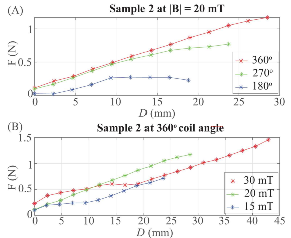
Figure 10: Results of grasping force characterization of VSR sample 2. Plots show the grasping force along the robot's -x axis ( F ) as a function of the linear displacement of the VSR ( D ) as the coiled robot is stretched along its x axis for: (A) coil deformation angles of 360^\circ , 270^\circ , and 180^\circ at a magnetic field of 20 mT, (B) coil deformation angle of 360^\circ at magnetic fields of 30 mT, 20 mT, and 15 mT.
