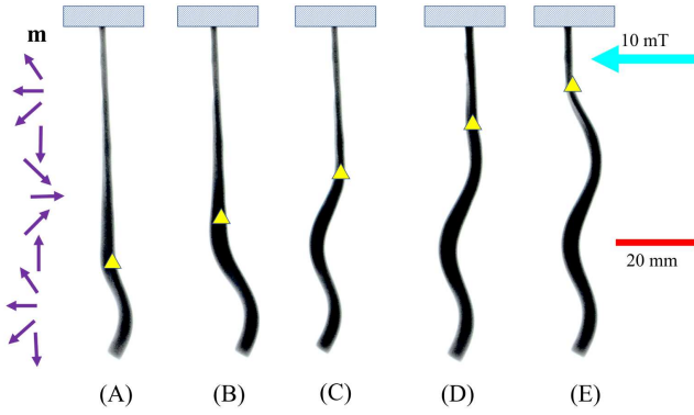
Figure 5: The variable stiffness robot (VSR), magnetized according to the purple arrows ( \mathbf{m} ) and constrained at the base (blue rectangles), is shown under static one-dimensional magnetic actuation (turquoise arrow) for various insertions of sliding nitinol backbone signified here by yellow triangles. (A) Distal 20 mm unconstrained. (B) Distal 30 mm unconstrained. (C) Distal 40 mm unconstrained. (D) Distal 50 mm unconstrained. (E) Distal 60 mm unconstrained. Due to the stiffness change factor, deformation can only occur in the unconstrained region of the VSR. This shows the lowest energy state of the sinusoidally magnetized VSR. When unactuated, the device (constrained or unconstrained) exhibits a straight profile being subject to only gravitational forces.
