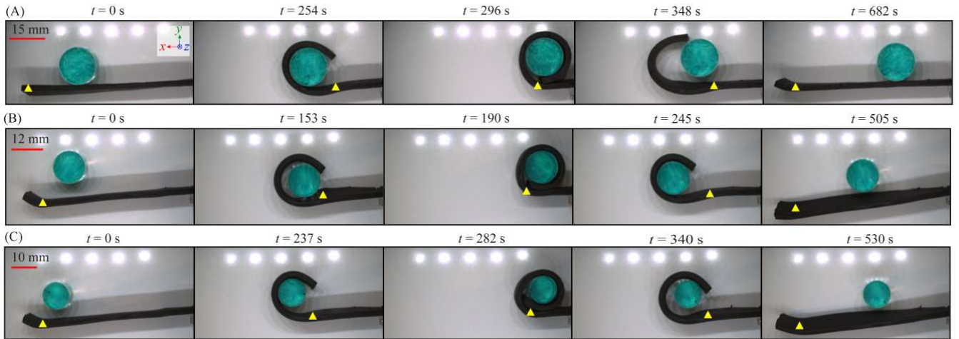
Figure 8: Closed-loop control demonstration of grasping and releasing objects placed at arbitrary locations and shown at different time instants ( t ) for three cases: (A) Sample 1 with 15 mm diameter object. (B) Sample 2 with 12 mm object. (C) Sample 2 with 10 mm object. The four stages of the experiment occur between the successive time snippets in the following order: grasping phase; coiling action; uncoiling action; releasing phase. The yellow triangle represents the tip position of the nitinol backbone. Please refer to the supporting video: S3-S5 for the complete demonstration.
