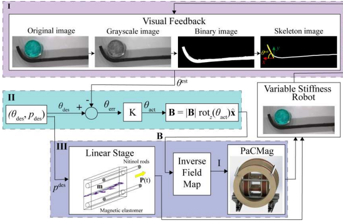
Figure 7: Closed-loop control of the variable stiffness robot (VSR) summarized in three blocks: (I) The tip angle ( \theta_{est} ) of the VSR is estimated from the camera and sent as feedback to the controller. (II) A proportional control calculates the magnetic field ( \mathbf{B} ) and its angle ( \theta_{act} ) to be applied from the error ( \theta_{err} ) between the desired ( \theta_{des} ) and estimated ( \theta_{est} ) tip angles. (III) PaCMag applies the magnetic field by computing the required current ( I ) from the inverse field map. The linear stage moves the nitinol backbone to a position ( p_{des} ) updated based on the current desired tip angle ( \theta_{des} ).
