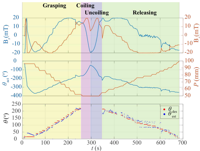
Figure 9: Results of closed-loop control experiment of Sample 1 grasping and releasing 15 mm object. Plots show the applied magnetic field ( B_x , B_y ) and its orientation ( \theta_{act} ), position of the nitinol backbone ( P ), the desired ( \theta_{des} ) and estimated ( \theta_{est} ) tip angles of the VSR during the experiment time ( t ). The four stages of the experiment occur as follows: grasping phase ( t = 0-254 s); coiling action ( t = 255-296 s); uncoiling action ( t = 297-348 s); releasing phase ( t = 349-682 s).
