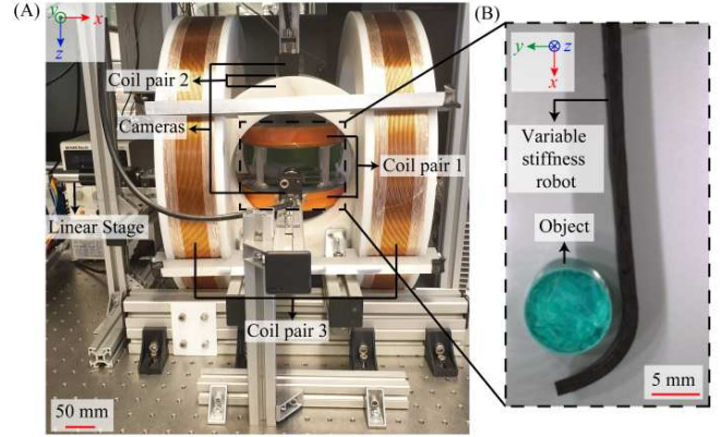
Figure 6: The actuation system showing (A) PaCMag - 3D electromagnetic coil setup and the linear stage. (B) Top view of the variable stiffness robot grasping an object in the workspace.
