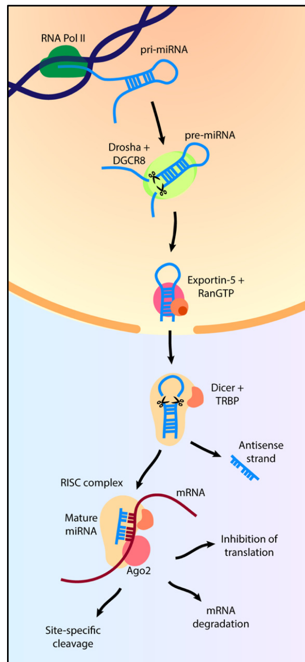
Figure 1. The canonical pathway of miRNA biogenesis.
