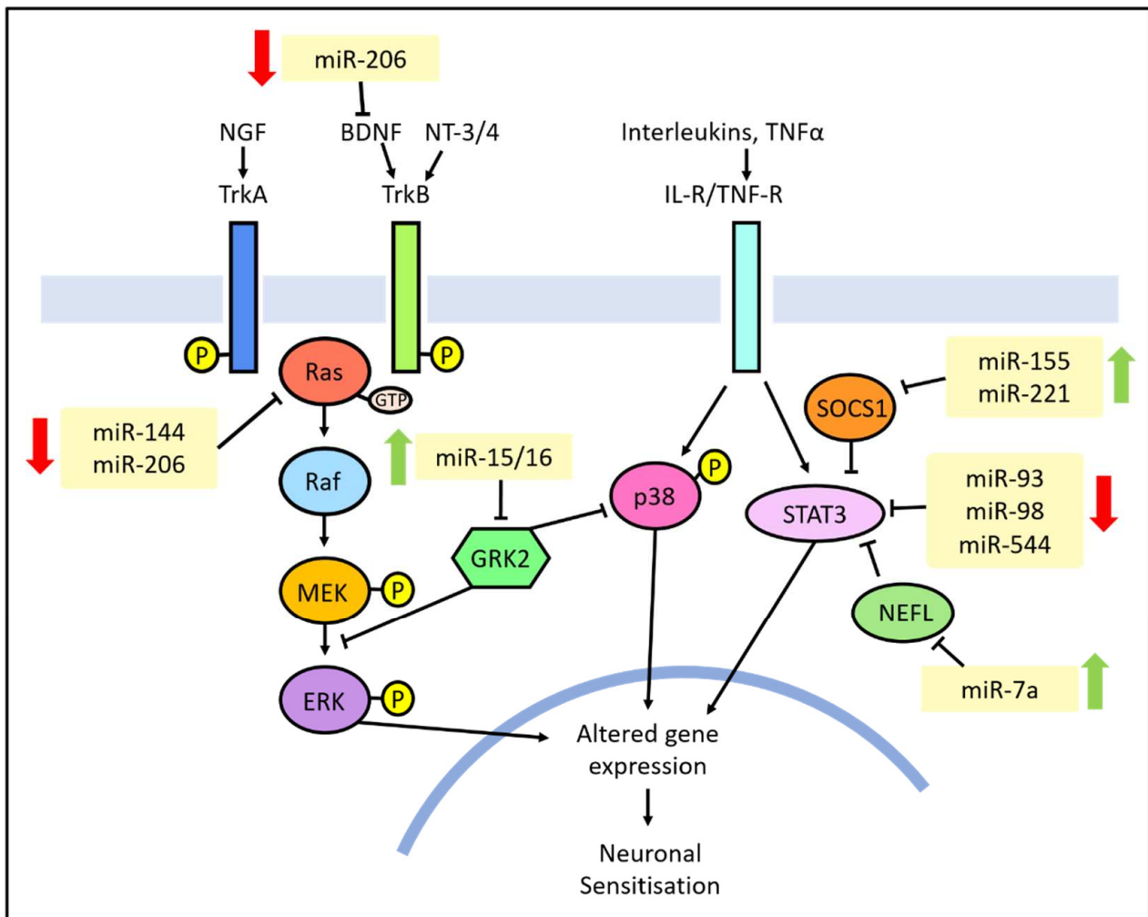
Figure 3. Diagram displaying miRNA dysregulated in neuropathic pain and their targets involved in intracellular signalling. Red downward arrows indicate that the miRNA is downregulated during neuropathic pain, whilst upward green arrows indicate miRNA upregulation in neuropathic pain.
