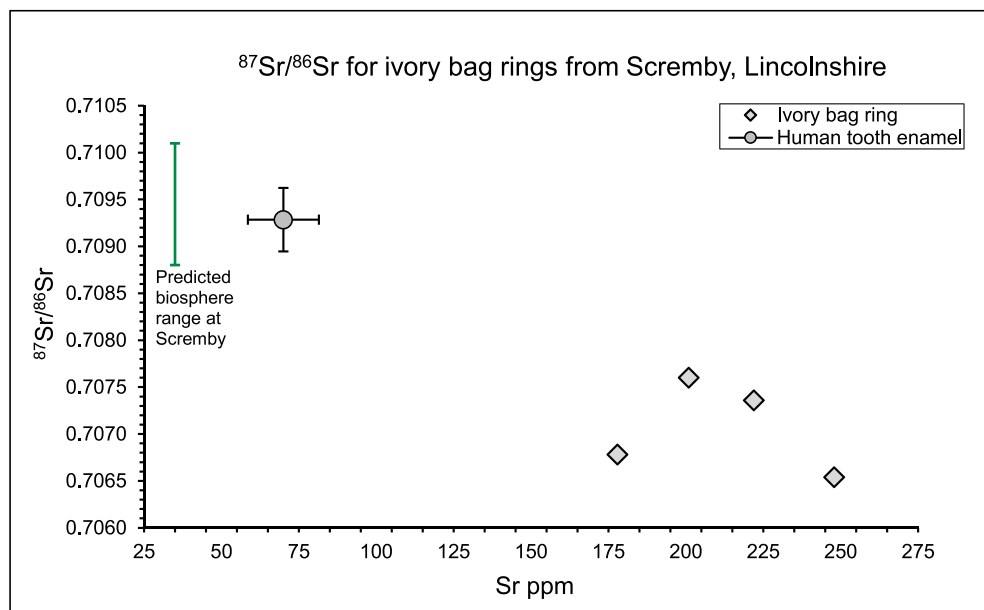
Fig. 6. Plot illustrating 87 Sr/ 86 Sr and strontium concentrations (ppm) for the ivory sampled from four bag rings associated with burials at Scremby, Lincolnshire (grey diamonds). The mean 87 Sr/ 86 Sr (0.7094 ± 0.0003, 1σ, n = 10,) and mean concentration (70 ppm ± 11.49, 1σ, n = 10) for human tooth enamel from Scremby is also represented by the grey circle, whilst the predicted biosphere range for the area is illustrated by a green bar. These data illustrate the difference between the values we expect for the local area and the 87 Sr/ 86 Sr of the sampled ivory (mean ivory 87 Sr/ 86 Sr: 0.7071 ± 0.0005, 1σ, n = 4; mean ivory concentration: 212 ppm ± 29.8, 1σ, n = 4). (For interpretation of the references to colour in this figure legend, the reader is referred to the web version of this article.)
