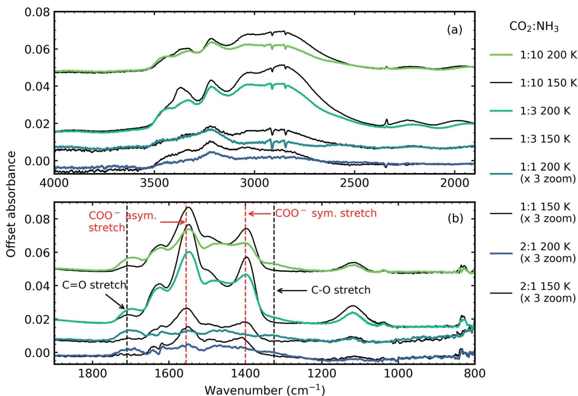
Fig. 5 Mid-IR spectra of \text{CO}_2 : \text{NH}_3 ices thermally processed to 150 K (black traces) and 200 K (coloured traces) (a) N–H and O–H stretching region ( 4000\text{--}1900\text{ cm}^{-1} ) and (b) 1900\text{--}800\text{ cm}^{-1} with dashed lines indicating \text{COO}^- asymmetric and symmetric stretches and C=O and C–O stretches. The 2 : 1 and 1 : 1 ratios have been magnified by a factor of 3 for clarity. All spectra are normalised to a thickness of 400 nm and offset on the y-axis for clarity.
