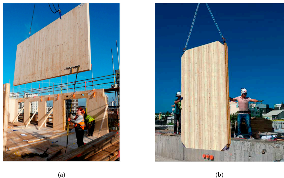
Figure 7. Panel lifting with (a) the conventional method [86] and (b) novel connectors (CLT-C2) [60].
