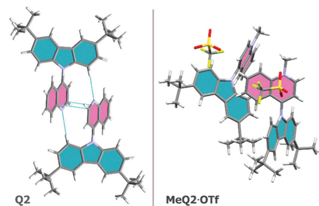
Fig. 7 Face-to-face aromatic intermolecular interactions in Q2 and their absence in MeQ2 -OTf from X-ray crystal packing.
