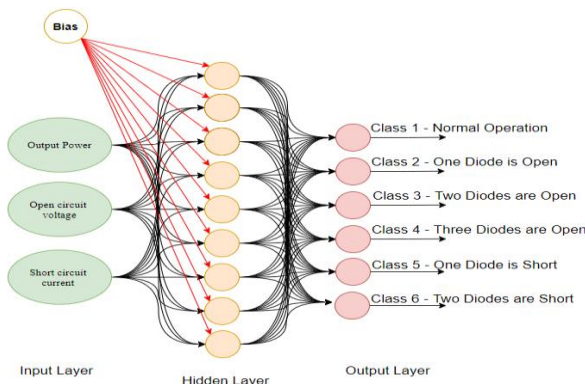
Fig. 4. Developed ANN model architecture.
