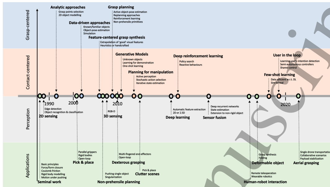
Figure 2. The figure shows the evolution of the robotic grasping and manipulation field. The research before early 2000 should be considered seminal work and primarily achieved with analytic approaches on a grasp-centered perspective. In 2008, the work in Saxena et al. [29] spawned the idea of looking for visual features for synthesizing grasp poses. The availability of depth sensors in 2009 introduced new 3D features. In early 2010, the paradigm switched to contact-centered grasping, which still dominates the field. Deep learning has revolutionized our perception capabilities and action-selection learning but at the cost of being data-inefficient. The late trend is to investigate more data-efficient methods such as one- or few-shot learning. Very recently, autonomous grasping and decision-making has been merged with HRI to combine users' cognitive abilities with reliable automation. In 2022, aerial transportation and payload stabilization have become extremely popular, catching the grasping community's attention.
