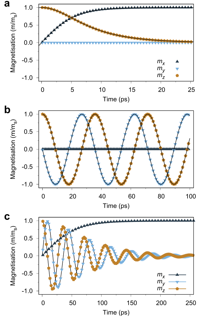
Figure 1. (a) Simulated time-dependent magnetisation for a single magnetic moment under the action of a pure relaxation torque B_{RT}^{\text{STT}} = 1.0\text{T} for initial conditions of \mathbf{m} = \hat{z} and polarization vector \mathbf{p} = \hat{x} (points). Lines show the analytical solution for the time-dependent dynamics. The dynamics show direct relaxation with a characteristic timescale \tau = 1/\gamma_e B_{RT}^{\text{STT}} . (b) Simulated time-dependent magnetisation for a single magnetic moment under the action of a pure precession torque B_{PT}^{\text{STT}} = 1.0\text{T} showing a continuous precessional motion around the polarisation vector \mathbf{p} . (c) Combined dynamics with B_{RT}^{\text{STT}} = 0.1\text{T} and B_{PT}^{\text{STT}} = -1.0\text{T} and zero external applied field showing standard LLG-like dynamics identical to a magnetic moment in a constant applied field of \mathbf{B}_{\text{app}} = 1.0\text{T} and \alpha_G = 0.1 . In general when the relaxation and precessional terms are included with no other terms LLG-like dynamics are exactly recovered for \alpha_G = B_{RT}^{\text{STT}}/B_{PT}^{\text{STT}} .
