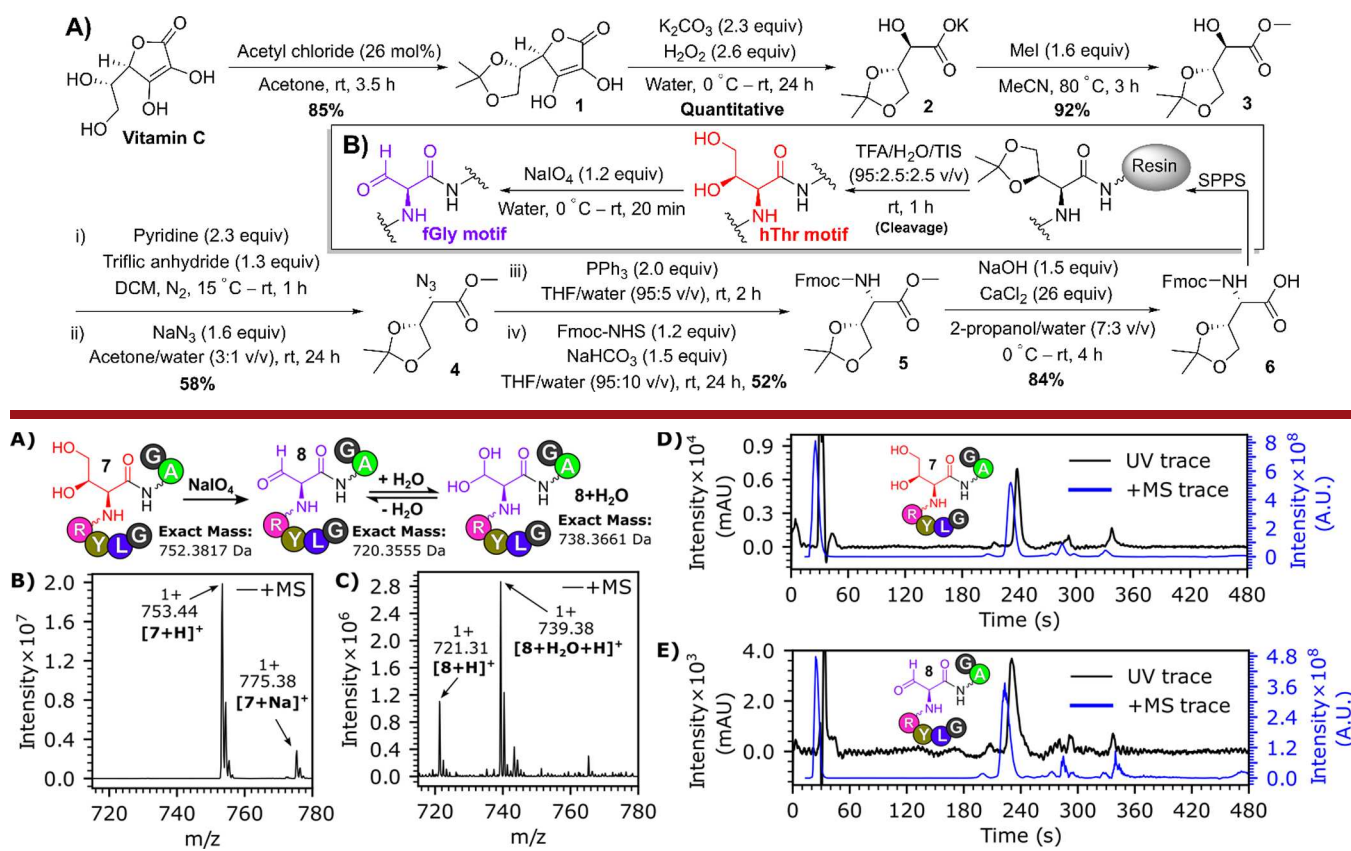
Figure 1. (A) Conversion of peptide 7 into peptide 8 using NaIO_4 . (B) MS analysis of 7 . (C) MS analysis of 8 . (D) LC-MS chromatogram of 7 . (E) LC-MS chromatogram of 8 . LC-MS chromatograms show the BPC+All MS trace and the UV chromatogram shows the absorbance for wavelengths 210–400 nm. LC-MS was conducted using LC gradient A (see Figure S1).
