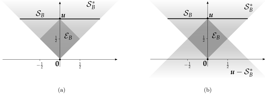
Figure 2: State and effect spaces S_B and E_B (the horizontal line and the dark square, respectively) of the classical-bit GPT system showing (a) the dual cone S_B^* (shaded) of the state space; (b) the effect space E_B is given by the intersection of the cones S_B^* and u - S_B^* since the bit is unrestricted (see Section 3.1).
