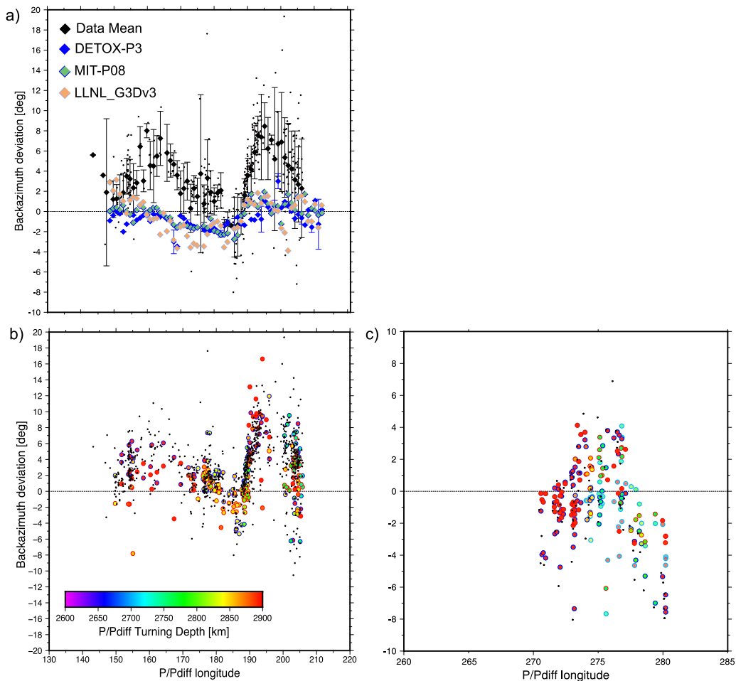
Fig. 7. Synthetic backazimuth deviations for different mantle velocity models. a) Comparison of backazimuth deviations from 3D tomographic velocity models for the synthetic dataset sampling the Pacific. Recorded backazimuth deviations are shown as black symbols with error bars. Symbol color indicates turning depths of the P -wave. b) Synthetic backazimuth deviations for the best fitting model for the Pacific region. Symbol color indicates turning depths of the P -wave. Recorded backazimuth deviations are shown as grey symbols. c) Synthetic backazimuth deviations for the best fitting model for the Gulf of Mexico. Recorded backazimuth deviations are shown as grey symbols. Symbol color indicates turning depths of the P -wave. Slow velocity model is indicated by symbols with black outlines and fast velocity model results are shown as symbols with thick blue outlines.
