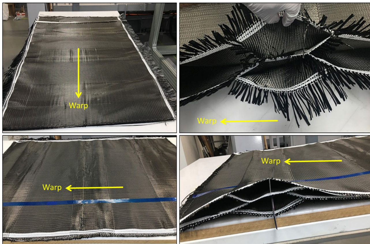
Figure 7. Samples of 3D woven honeycomb fabric.
