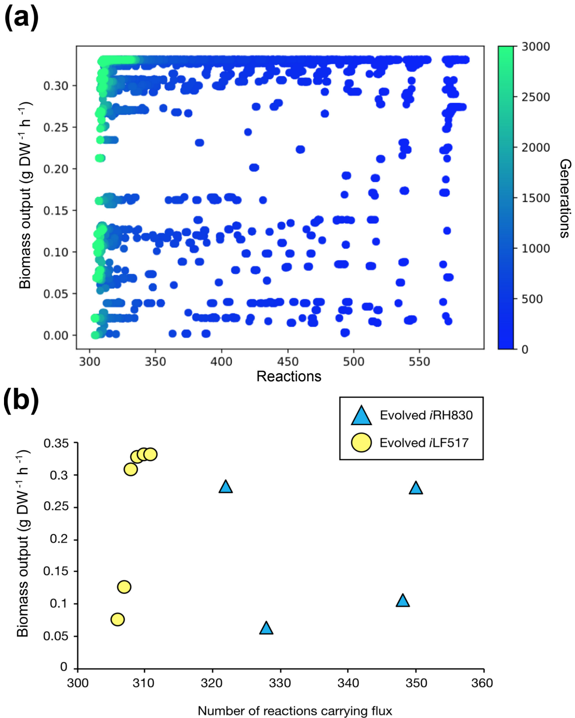
Fig. 7. Evolution of iLF517 . (a) Evolution of iLF517 in a blood medium. MOEA was run for 3000 generations (blue to green). (b) Biomass output [g DW (mmol glucose) -1 h -1 ] and the number of reactions carrying flux in evolved iRH830 (blue triangles) and evolved iLF517 (yellow circles) models. The evolved solutions produce comparable biomass outputs. Ten evolved solutions are given for each, some duplicates are present.
