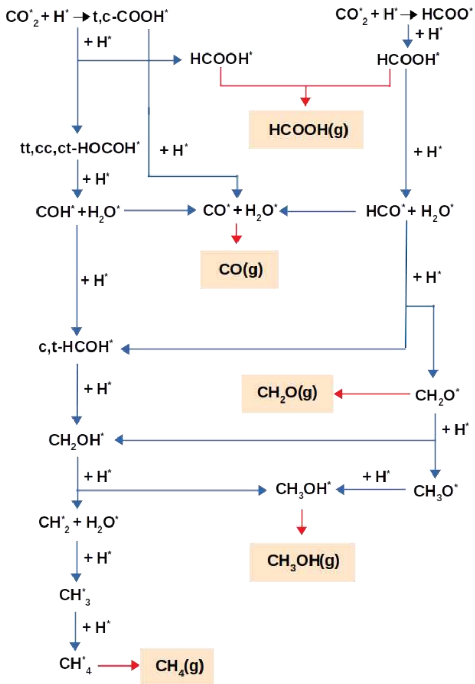
Figure 2. Possible CO 2 hydrogenation reaction mechanisms on the NbC (111) surface.
