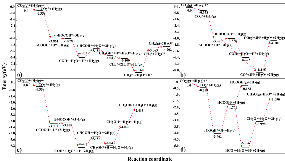
Figure 6. The preferred reaction profiles for \text{CO}_2 hydrogenation to a) \text{CH}_4 , b) \text{CO} , c) \text{CH}_3\text{OH} , and d) \text{CH}_2\text{O} and \text{HCOOH} on the NbC (111) plane. The illustrated profiles are compared to the summation of the total free energies of the catalyst, \text{CO}_2 , and four \text{H}_2 in the gas phase 46 .
