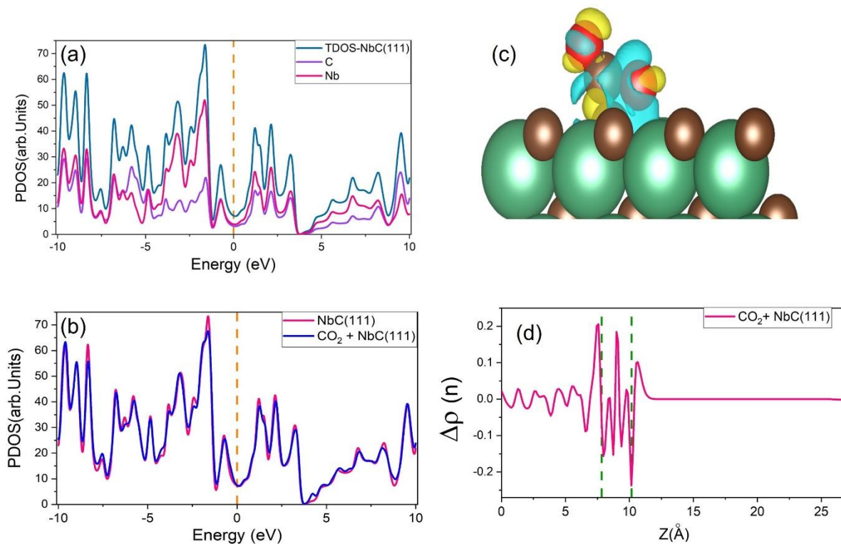
Figure 4. a) The PDOS for NbC (111) surface, b) The TDOS of NbC (111) prior and after adsorption of CO 2 , c) The charge density differences inside view, the C and O atoms illustrated in brown and red (isovalue= ±0.002) and, d) The planar average charge density. The Fermi level is set at zero.
