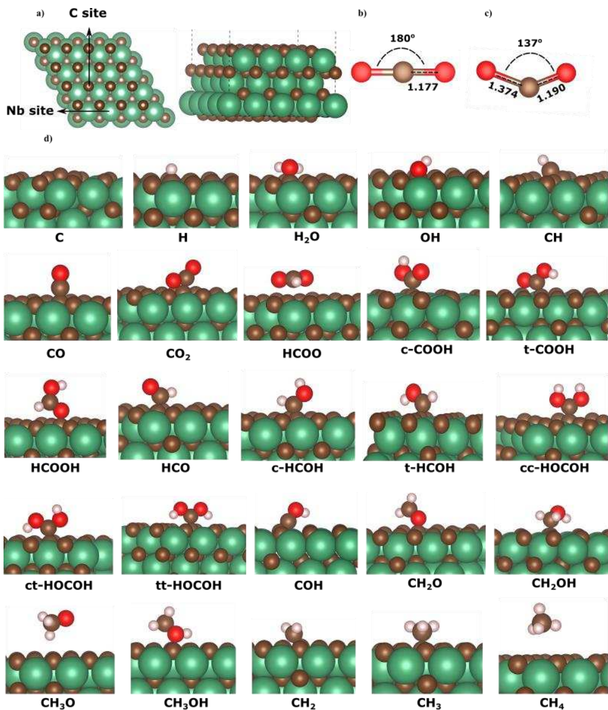
Figure 1. a) The NbC (111) plane, isolated CO 2 molecule b) prior, c) following adsorption and, d) adsorption structures with minimal energy for all intermediates on the NbC (111) plane.
