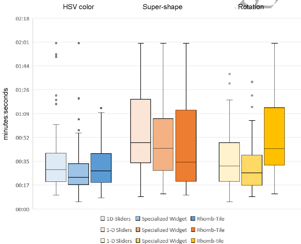
Figure 12. Task completion times for the considered 3-D parameter domains. Markings of the box plots correspond to minimum, interquartile range, mean, and maximum. Individual points correspond to outliers.
