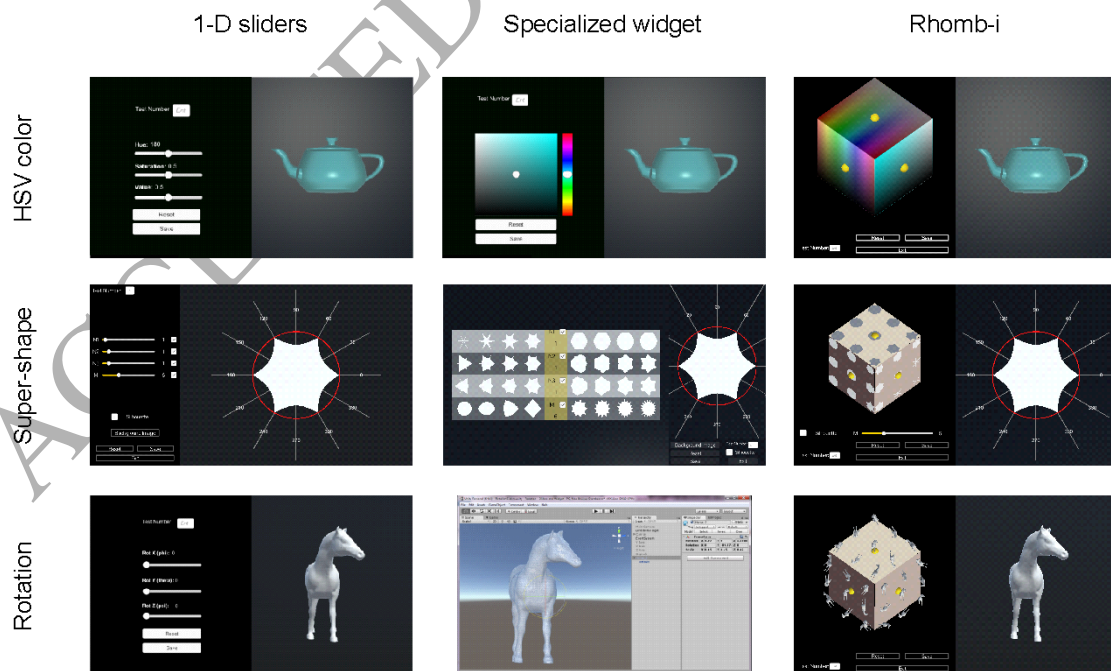
Fig. 10. User tasks for exploring 3-D parameter domains.
