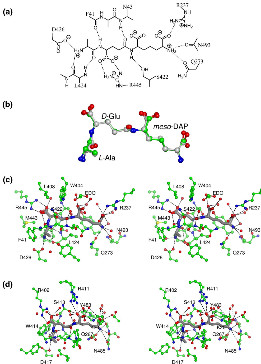
Fig. 4. Mode of murein tripeptide binding in DppE. (a) Schematic representation of the polar interactions (dashed lines) between DppE and the murein tripeptide ligand. (b) Superposition of the murein tripeptide ligands from the crystal structures of DppE from B. subtilis and MppA from E. coli . The colouring is by atom type: oxygen, red; nitrogen, blue; carbon, green in DppE and grey in MppA. (c and d) Stereo images illustrating the interactions of murein tripeptide shown in cylinder format (grey carbons) and the residues of the binding pocket shown in ball-and-stick format (green carbons). Polar interactions of the Mtp ligand and the surrounding protein and water molecules (red spheres) are indicated by dashed lines. In (c), EDO refers to ethane diol introduced during crystal cryoprotection.
