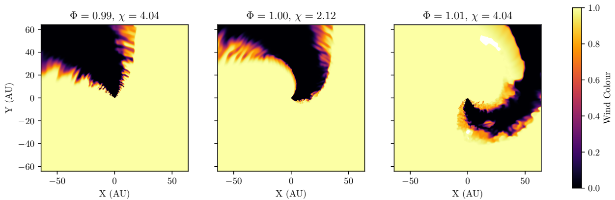
Figure 8. Wind “colour” in a simulation of the WR140 system shortly before, during, and after periastron. A colour of 1 represents a pure WR wind and a colour of 0 represents a pure OB wind. We find that the wind undergoes more mixing during and after periastron.
