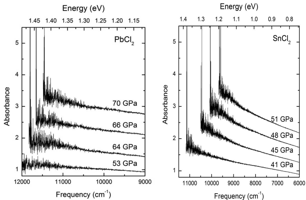
FIG. 10. Representative high-pressure spectra of the absorption edge of \text{PbCl}_2 (a) and \text{SnCl}_2 (b). No exciton peaks are resolved within these experiments. These spectra show that the energy of the band gap decreases as pressure increases . Spectra are stacked for clarity.
