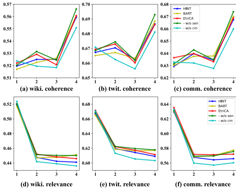
Figure 6: The results of intra-story coherence and relevance on the ROC dataset.
