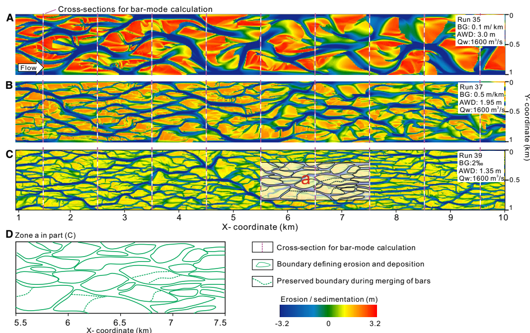
Fig. 7. Bar morphology in modelled braided rivers with varying bed gradients and fixed discharge (1600 m 3 /s). AWD, average water depth; BG, bed gradient; Qw, flow discharge. (A) to (C) Maps of riverbed erosion and sedimentation produced by different runs, with bed gradients of 0.1 m/km, 0.5 m/km and 2.0 m/km, respectively. (D) Bar boundaries extracted from the part of map corresponding to Zone A in part (D).
