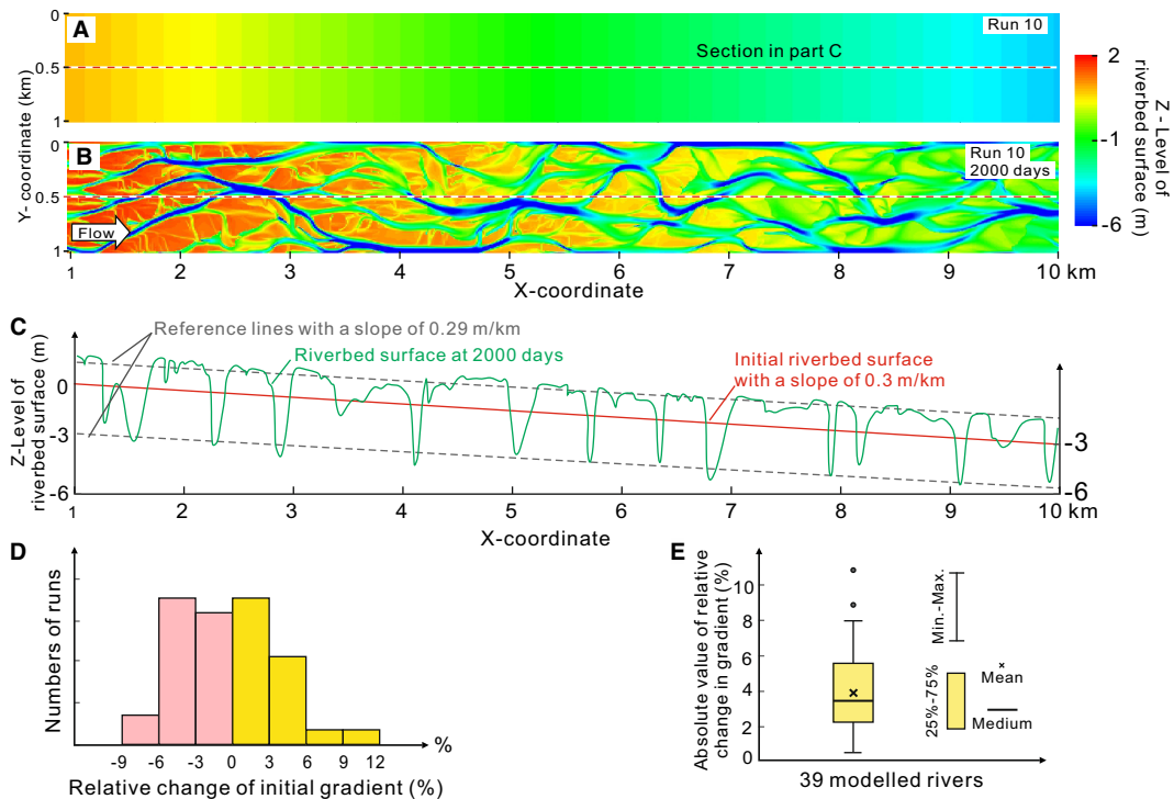
Fig. 6. Riverbed gradient characteristics. (A) Initial riverbed surface level with a gradient of 0.3 m/km. (B) Riverbed surface level at 2000 days, with a gradient of 0.29 m/km; this refers to the example shown in Fig. 3E. (C) Comparison between the riverbed surface at 0 days and 2000 days; section location is shown in part (A). (D) Histogram showing the frequency distribution of changes in riverbed experienced by the 39 modelled rivers. (E) Box plot showing the absolute values of changes in gradient, expressed relative to the initial gradient, for the 39 model runs.
