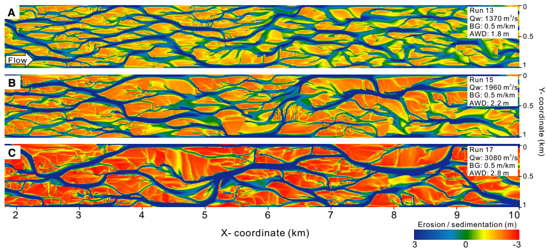
Fig. 9. Bar morphology in braided rivers with the same bed gradient but variable discharge. (A) to (C) Maps of riverbed erosion and sedimentation for runs in which the river slope is 0.5 m/km, and the discharge values are 1370 m 3 /s, 1960 m 3 /s and 3080 m 3 /s, respectively, corresponding to average water depths of 1.8 m, 2.2 m and 2.8 m, respectively. AWD, average water depth; BG, bed gradient; Qw, flow discharge.
