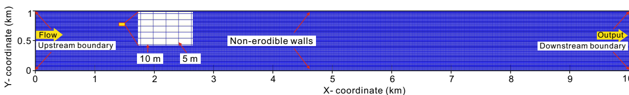
Fig. 2. Boundary and grid setting of the braided-river model (plan view). The upstream and downstream boundaries of the model, and the direction of river flow, are indicated. The model grid is bounded by non-erodible walls. Grid-cell size is 10 m along X (downstream) and 5 m along Y (cross-stream).
