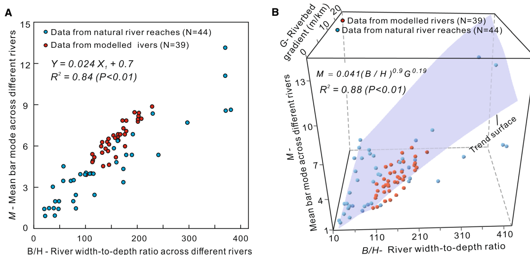
Fig. 12. Relationships between bar mode and river characteristics. (A) Mean bar mode versus river width-to-depth ratio across 44 real-world river reaches and the 39 modelled rivers. (B) Cross-plot of bar mode versus river width-to-depth ratio and riverbed gradient, across 44 real-world river reaches and the 39 modelled rivers. R^2 is the coefficient of determination; regressions are statistically significant at P = 0.01 (two-tailed). The underlying data are provided in Tables S1 to S3; see Supplementary Information.
