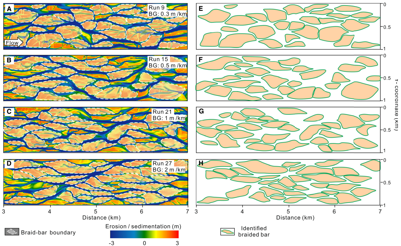
Fig. 10. Bar morphology in braided rivers with variable slope but the same average water depth across different runs. River flow is from the left for all the modelled rivers. The mean channel depths are similar, varying between 7.0 to 7.2 m. (A) to (D) Maps of riverbed erosion and sedimentation for runs in which the gradient increases as follows: 0.3 m/km, 0.5 m/km, 1.0 m/km and 2.0 m/km. (E) to (H) Outlines of the braid bars identified in the corresponding maps (parts A to D). BG, bed gradient.
