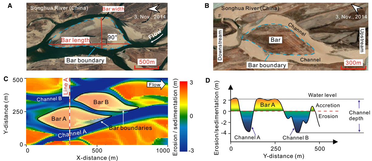
Fig. 1. Practical approach followed for placing the boundary between bars and channels. (A) Aerial photograph of the Songhua River, China ( 45^{\circ}13'59''\text{N} , 43^{\circ}10''\text{E} ), at low flow stage. (B) Aerial photograph of the Songhua River, China ( 45^{\circ}3'25''\text{N} , 124^{\circ}59'21''\text{E} ), presenting a mid-channel bar adjacent to channels with dry beds. Sandy channel beds are lighter coloured, whereas the vegetated bar appears darker. (C) Map of the amount of erosion and sedimentation of the riverbed of a modelled river, relative to the initial planar surface. The boundaries of two bars (labelled as 'Bar A' and 'Bar B') are shown as examples. (D) Cross-section of Line A in part (C).
