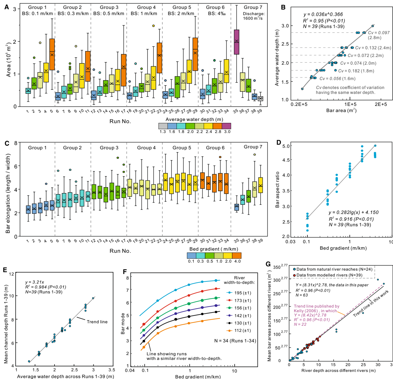
Fig. 11. Statistics relating bar geometry to model characteristics and boundary conditions for 39 simulation runs. The total number of measured bars is 1400. R is the Pearson's correlation coefficient; correlations are statistically significant at P = 0.01 (two-tailed). Cv denotes the coefficient of variation of bar areas for the same values of average water depth. (A) Box plots of bar areas. Model runs in each of groups 1 to 6 have the same initial bed gradient; runs in group 7 have the same water discharge. (B) Mean bar areas versus average water depth. Different runs in which the same average depth emerges show similar values of bar area, indicated by the small coefficients of variation. (C) Box plots of values of bar aspect ratio. (D) Mean values of bar aspect ratio versus river gradient. (E) Mean channel depth (river depth) versus average water depth (raster mean) for the 39 runs. (F) Bar mode versus bed gradient in different river width-to-depth ratios. (G) River depth versus mean bar area across 39 modelled rivers and 24 real-world rivers. The trend line between river depth and mean bar area proposed in this work is compared to that reported by Kelly (2006).
