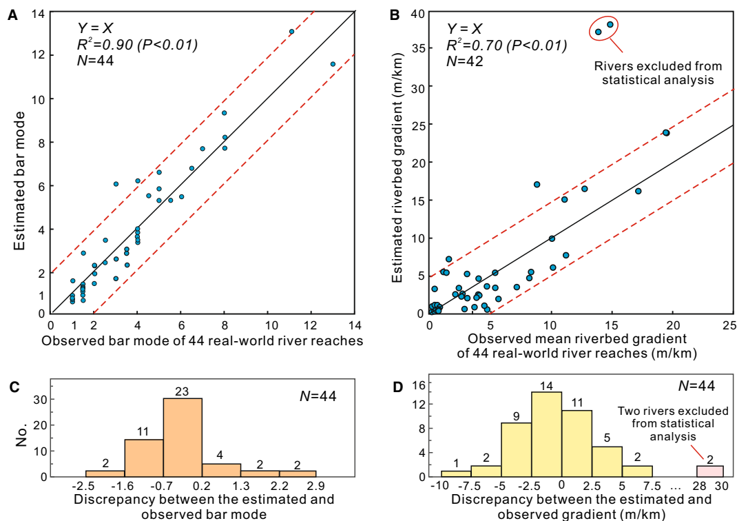
Fig. 13. Analysis of bar-mode and riverbed-gradient predictions. (A) Cross-plot of bar mode estimated using Eq. 5 versus observed bar mode for 44 real-world river reaches. (B) Cross-plot of riverbed gradient estimated using Eq. 7 versus observed riverbed gradient for 44 real-world river reaches; gradient estimations of two rivers (red ellipse) were excluded in the analyses as they are regarded as outliers. (C) Histogram displaying the discrepancy between estimated and observed values of bar mode. (D) Histogram displaying the discrepancy between estimated and observed river gradient. The underlying data are provided in Tables S1 and S2; see Supplementary Information.
