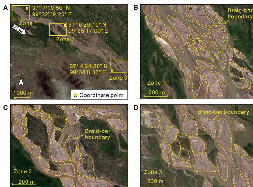
Fig. 8. Satellite images of a reach of the Buha River, China, illustrating that bar aspect ratio tends to increase with increasing river slope. (A) Overview. (B to D) River reaches corresponding to Zone 1, Zone 2 and Zone 3 in part (A), respectively, which have slopes of approximately 3.5 m/km, 1.9 m/km and 1.4 m/km, respectively.
