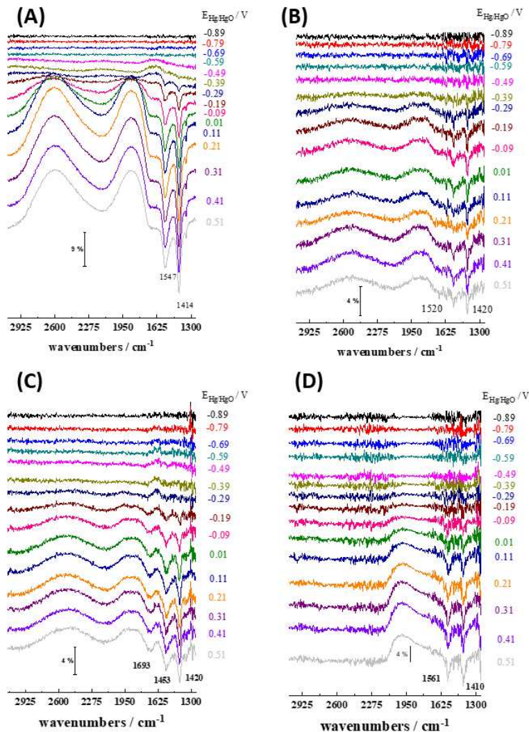
Fig. 3 FTIR spectra for EOR 0.5 M EtOH in 0.5 M KOH/H 2 O recorded between -0.89 V and 0.51 V at 1 mVs -1 for A)Pd/C SBIPA , B)PdAuNi/C 3steps , C)PdAuNi/C SBEG and D)PdAuNi/C SBIPA
