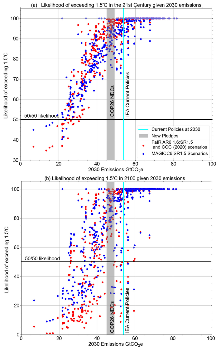
Figure 1. Likelihood of (a) peak or (b) 2100 temperature exceeding 1.5°C versus 2030 emissions. We show MAGICC6 simulations (blue dots) and FaIR AR6 simulations (red dots) using the period 2011–2020 to define the observed warming since the pre-industrial period. Scenarios are from the SR15 database complemented with additional runs from the Committee on Climate Change. Highlighted is the Climate Action Tracker assessment of 2030 nationally determined contribution emissions and the current 2030 emissions from International Energy Association (IEA) given pre-COP26 stated policies. There are 134 scenarios when run with FaIR and 100 for MAGICC with a 100% likelihood of exceeding 1.5°C in this database for both (a) peak warming and (b) 2100 temperatures.
