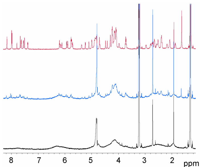
Figure 6. Time dependence of B-DNA NMR spectrum.
