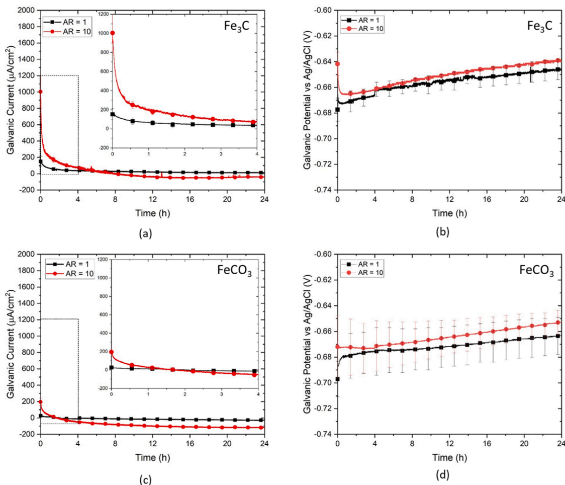
Fig. 7. (a, c) ZRA galvanic current and (b, d) galvanic potential measurements over 24 h at AR = 1:1 and AR = 10:1 in a CO 2 -saturated, pH 5, 1 wt% NaCl solution at 50 °C obtained by coupling a wet ground X65 carbon steel coupon to (a, b) an Fe 3 C-layered carbon steel coupon and (c, d) an FeCO 3 -layered X65 carbon steel coupon. The dashed rectangle shows the area magnified in the inset plots.
