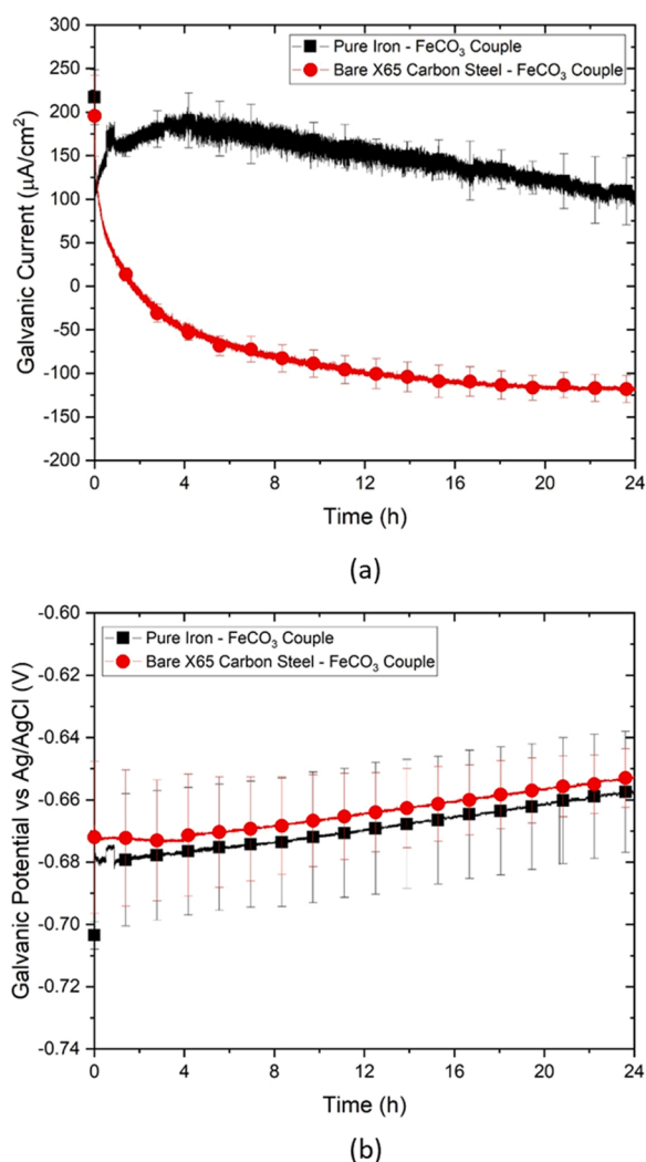
Fig. 11. Comparison of galvanic current and galvanic potential measurements in a CO 2 -saturated, pH 5, 1 wt% NaCl solution at 50 °C for a wet ground pure iron coupon coupled to an FeCO 3 -layered coupon and wet ground X65 carbon steel coupled to an FeCO 3 -layered coupon at AR = 10:1.
