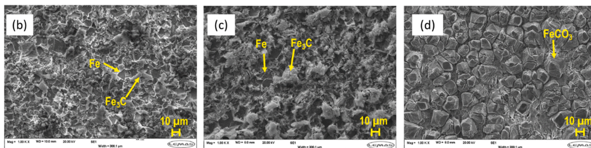
Fig. 5. (a) Corrosion rates, determined from LPR measurements, of bare X65 carbon steel and layered coupons in a CO 2 -saturated, pH 5, 1 wt% NaCl solution at 50 °C and top-view SEM images after 24 h exposure of (b) bare X65 steel, (c) an Fe 3 C-layered X65 steel coupon and (d) an FeCO 3 -layered X65 steel coupon.
