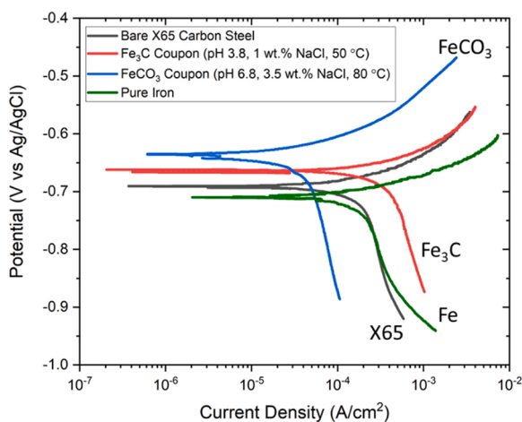
Fig. 6. Potentiodynamic polarisation plots measured after 15 min of immersion in a pH 5, CO 2 -saturated 1 wt% NaCl solution at 50 °C of a wet ground X65 carbon steel coupon, a wet ground pure iron coupon, an Fe 3 C-layered X65 carbon steel coupon and an FeCO 3 -layered X65 carbon steel coupon.
