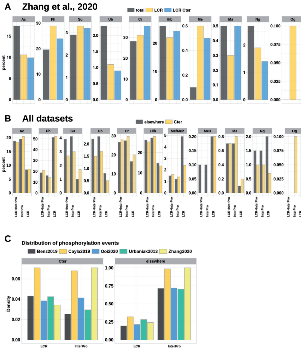
Figure 10. Mapping of post-translational modifications. A) The relative representation (percent) of post-translational modifications, identified in T. brucei bloodstream parasites by Zhang et al. 14 , were analysed in the total proteome (grey), in the low-complexity regions (LCRs; yellow) or in the LCRs located in the C-terminal region of their corresponding protein (blue). B) The Zhang et al. dataset 14 was merged with those obtained by: Urbaniak et al. , 2013, Benz et al. , 2019, Cayla et al. , 2019, Ooi et al. , 2020 for the analysis of phosphorylation, Fisk et al. , 2013 and Lott et al. , 2013 for the mono/di-methylation and Moretti et al. , 2018 for the lysine acetylation 13-16,18-20,31 , to obtain the positions of all documented modifications. The relative representation (percent) of post-translational modifications was analysed in the InterPro domains + LCRs, InterPro domains only or LCRs only, according to the position within the domain/LCR on which they are located, i.e. C-terminal (yellow) or elsewhere (grey). The distributions of phospho-residues were compared between the different datasets for their position within domains/LCRs, according to the position of the domain/LCR on which they are located: C-terminal or elsewhere. C) Density distribution of the phosphorylation event from the different datasets.
