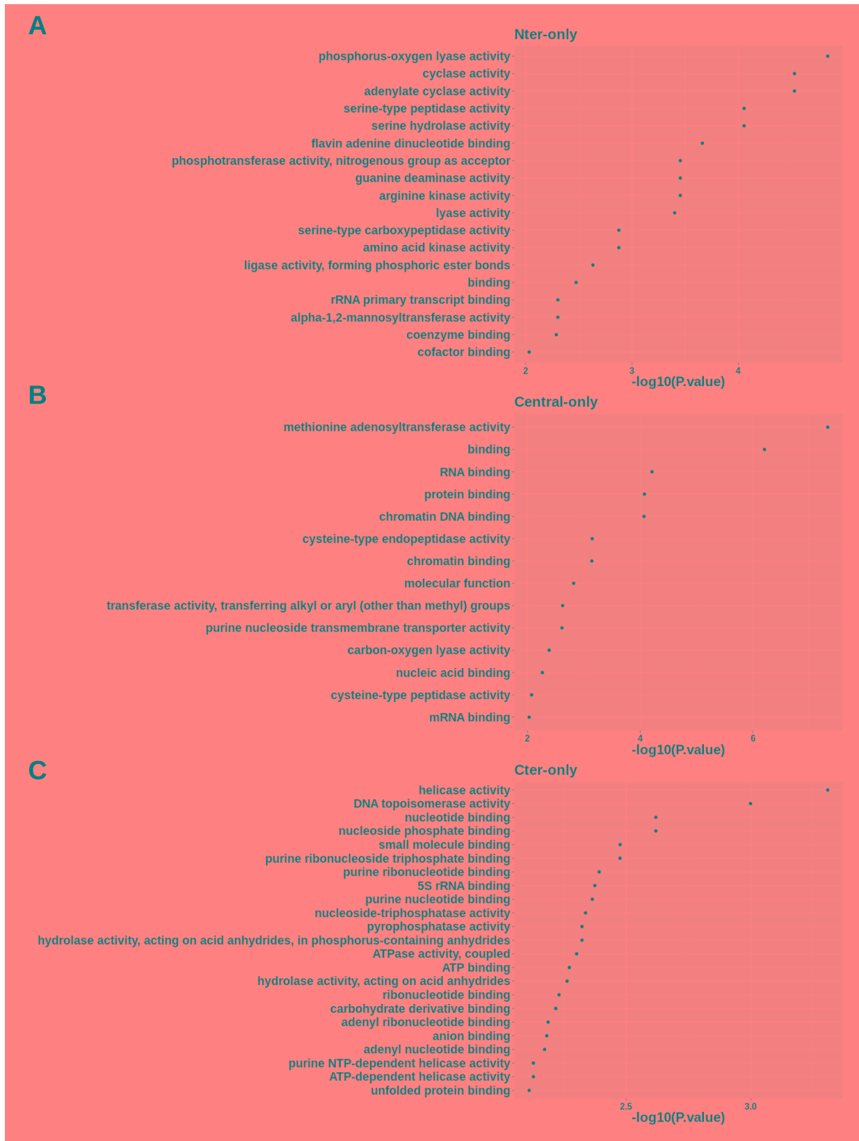
Figure 6. Graphical representation of the -\log_{10} of the p-value obtained with the molecular function Gene Ontology (GO) term analysis for proteins that possess low-complexity regions (LCRs) either only located in their N-terminal ( A ), Central ( B ) or C-terminal ( C ) part.
