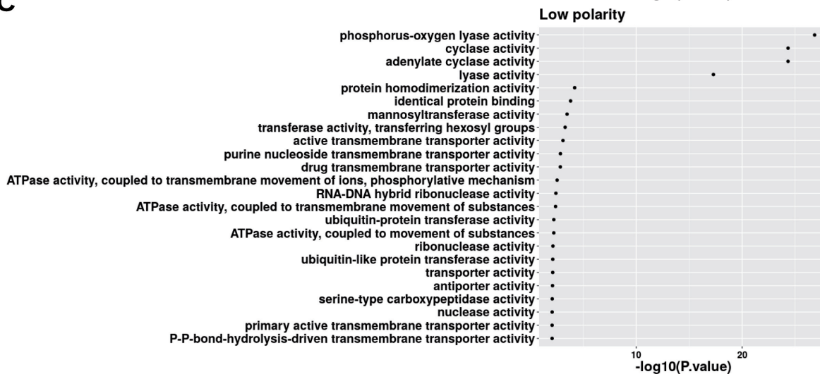
Figure 8. Graphical representation of the -\log_{10} of the p-value obtained with the molecular function Gene Ontology (GO) term analysis for proteins that possess low-complexity regions (LCRs) of either High (A), Intermediate (B) or Low (C) polarity indices.
