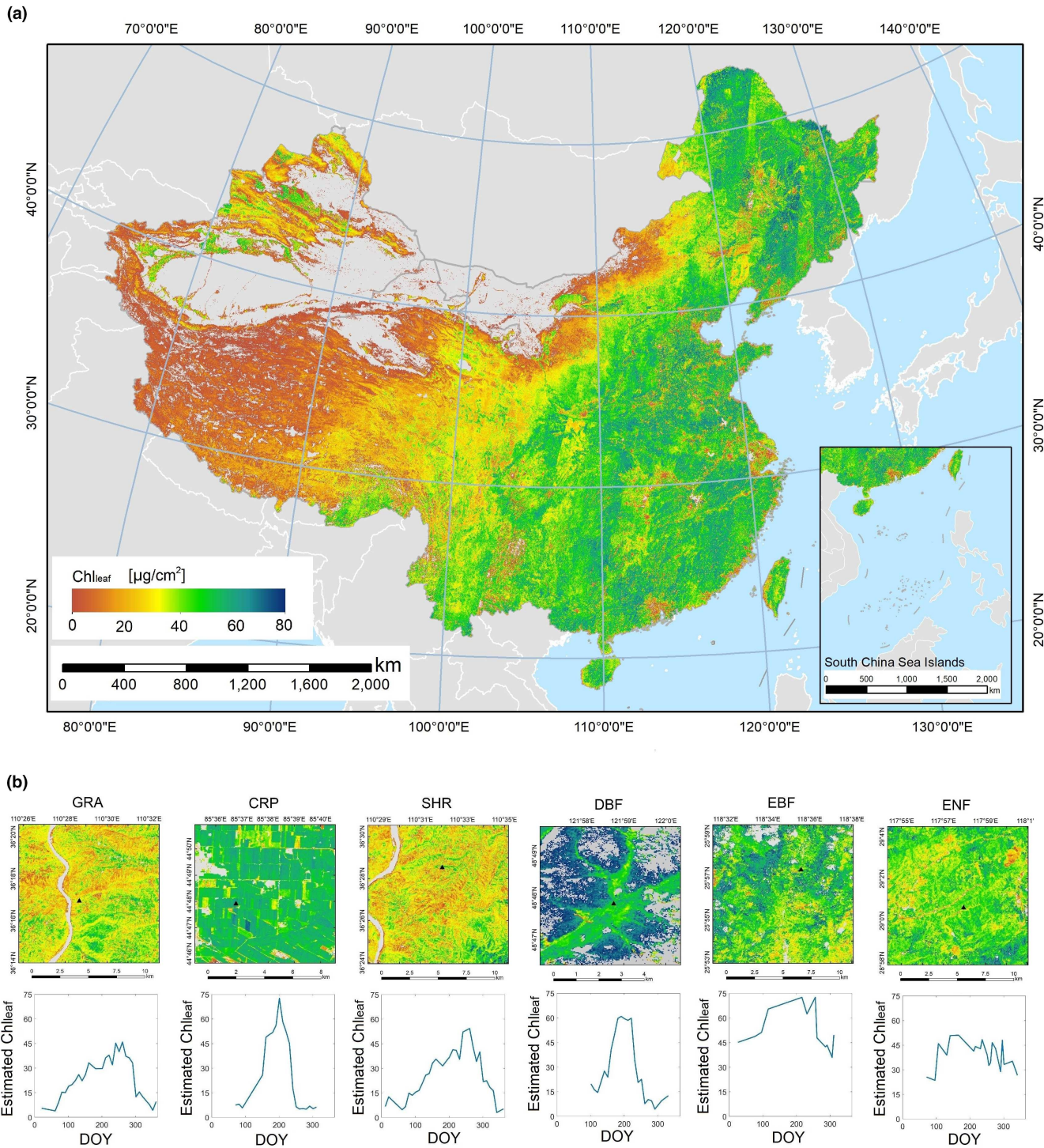
FIGURE 9 (a) Map of Ch_{leaf} across China. In addition to the regression models in Table 4, the Ch_{leaf} of SHR was calculated using Ch_{leaf} = 130.34 \cdot CSI - 25.37 (RMSE = 10.21 \mu g cm^{-2} , R^2 = 0.88 ). (b) Ch_{leaf} product images on July 2019 and the seasonal variation for each type.
