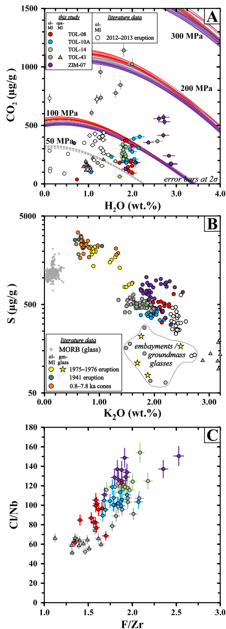
Fig. 6. [A] \text{H}_2\text{O} – \text{CO}_2 concentrations measured in the melt inclusion glasses in this study, and melt inclusions of the 2012–2013 eruption (Plechov et al. , 2015). Saturation isobars for all melt inclusions from samples TOL-16-08 (red curves), TOL-16-43 (grey curves; dotted = cpx-hosted inclusions), and ZIM-16-07 (purple curves) were computed at the specified pressure using VESical (v. 0.1.8; Iacovino et al. , 2021; Wieser et al. , 2021) with the MagmaSat model (Ghiorso & Gualda, 2015) at 1000°C for olivine-hosted inclusions and 900°C for clinopyroxene-hosted inclusions. [B] Melt inclusion S concentration vs \text{K}_2\text{O} (errors on new melt inclusion data are smaller than symbol). Note that logarithmic Y-axis and highlighted group of embayments/groundmass glasses with relatively low S contents. MORB array data from Jenner & O'Neill (2012) and Reekie et al. (2019) with MORB glasses filtered at \text{K}_2\text{O} \leq 0.4 wt.%. [C] Melt inclusion Cl/Nb vs F/Zr relationship, again showing tightly clustered data for each cone, and differences between the olivine- and clinopyroxene-hosted inclusions from sample TOL-16-43. Overall, melt inclusions from ZIM-16-07 show the highest Cl, F, S, and \text{H}_2\text{O} contents of all the samples analysed.
