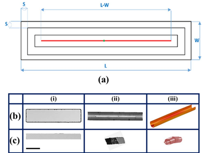
Figure 3. (a) Schematic view of the isotropic etching process. (b) and (c) demonstrate the effects of the aspect ratio on the rolling behavior. At (b), L/W = 4 , and C/W = 1.4 ; and at (c) L/W = 8 , C/W = 2.8 . (i) and (ii) are the images of the ribbon from experiments before and after releasing, respectively, and images at (iii) are the corresponding simulation results (scale bar size is 200 \mu\text{m} ).
