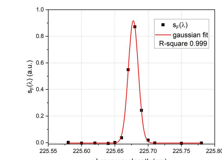
Wavelength scan of fluorescence signal integrated over x , t for O
