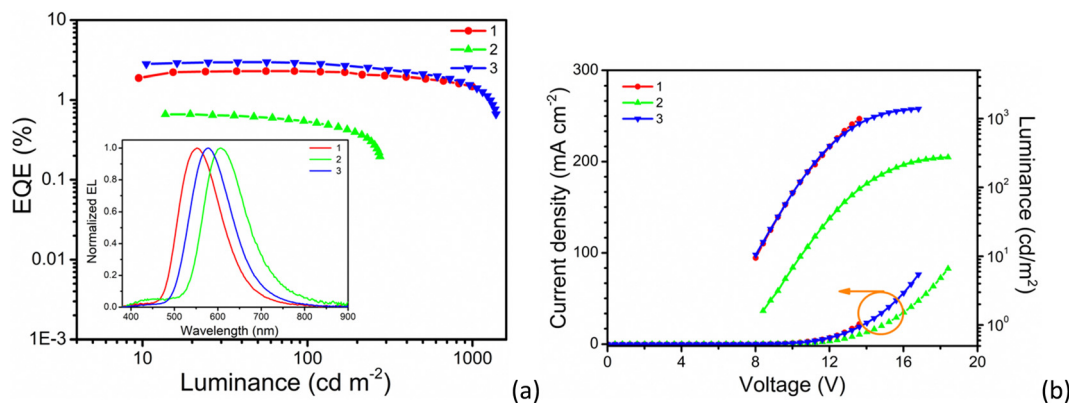
Fig. 8 Device performance at 1 wt% dopant concentration: (a) EQE-luminance curves (inset: the EL spectra); (b) J - V - L curves.
