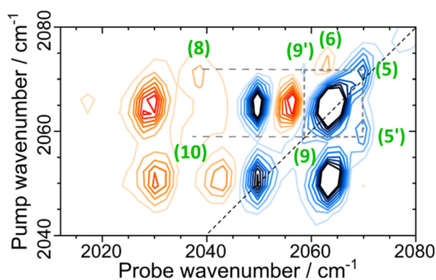
Fig. 7 2D-IR spectrum of EcHyd-1 at T_w = 250 fs in the \nu_{\text{CN}} region of the spectrum, with full peak assignment for the minor set (dashed lines) of coupled CN modes due to the \text{Ni}_\text{r}\text{-S}_{\text{I/II}} state.
