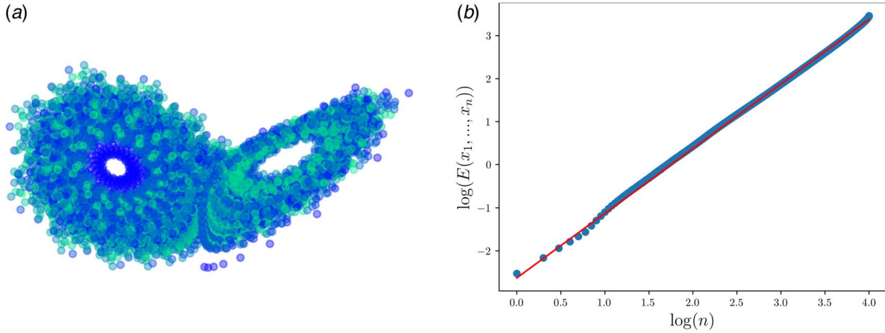
Fig. 6 Lorenz attractor: (a) dense Lorenz attractor and (b) log-log plot to determine fractal dimension, with gradient
