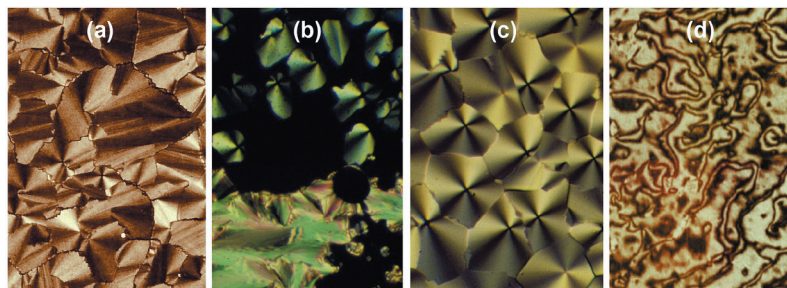
Figure 6. (Colour online) Photomicrographs of the mesophases of 4-decyloxybiphenyl-cyanobenzoate (10OBCB) \times 100 ; (a) the texture of the \text{Sm } \tilde{\text{C}} phase formed from the SmA phase, (b) the formation of the \text{Sm } \tilde{\text{C}} phase in the homeotropic area of the SmA phase on cooling, (c) the texture of the columnar phase of 10OBCB, note the lack of focal-conic defects, and (d) the schlieren texture of the SmC phase formed on cooling the \text{Sm } \tilde{\text{C}} phase.
