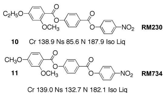
Figure 13. The structures and phase transitions (°C) of compounds RM230 and RM734.
